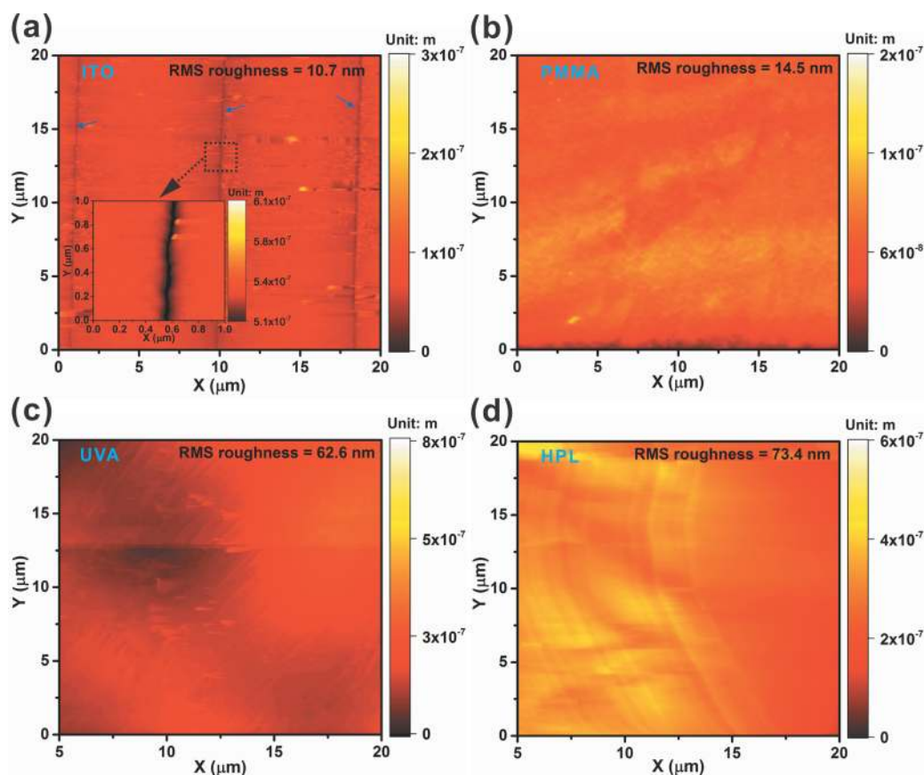
Figure 5. AFM maps of (a) ITO, (b) PMMA-transferred graphene, (c) UVA-transferred graphene, and (d) HPL-transferred graphene on PET after 10^4 bending cycles.
