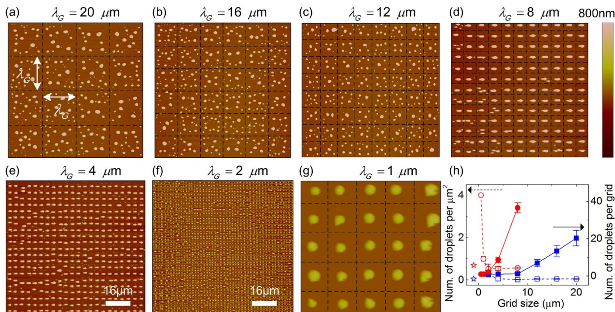
Figure 5 | (a)–(g) provide the dewetting results for a film with \sim 26 nm initial thickness. The size of cutting grid, \lambda_G changes from 20 \mu\text{m} to 1 \mu\text{m} . The dashed lines represent mechanically modulated locations, which are not shown in (e) and (f) due to large droplets density. The mean diameters of the dewetted droplets for \lambda_G = 20, 16, 12 \mu\text{m} are 1.10, 1.11, 1.09 \mu\text{m} , respectively; the corresponding standard deviation for these mean diameters are 0.64, 0.61, 0.57 \mu\text{m} , respectively. The diameter data for \lambda_G = 8, 4, 2 \mu\text{m} corresponds to the case of R = 66\% in Figure 6. (h) plots the number of droplets per \mu\text{m}^2 (dashed lines) or the number of droplets per grid (solid lines) and grid size for h_0 \sim 26 nm (rectangular) and h_0 \sim 12 nm (circle). Data marked by open markers correspond to the number of droplets per \mu\text{m}^2 for uncontrolled area. The dewetted results for h_0 \sim 12 nm are shown in Figure 7.
