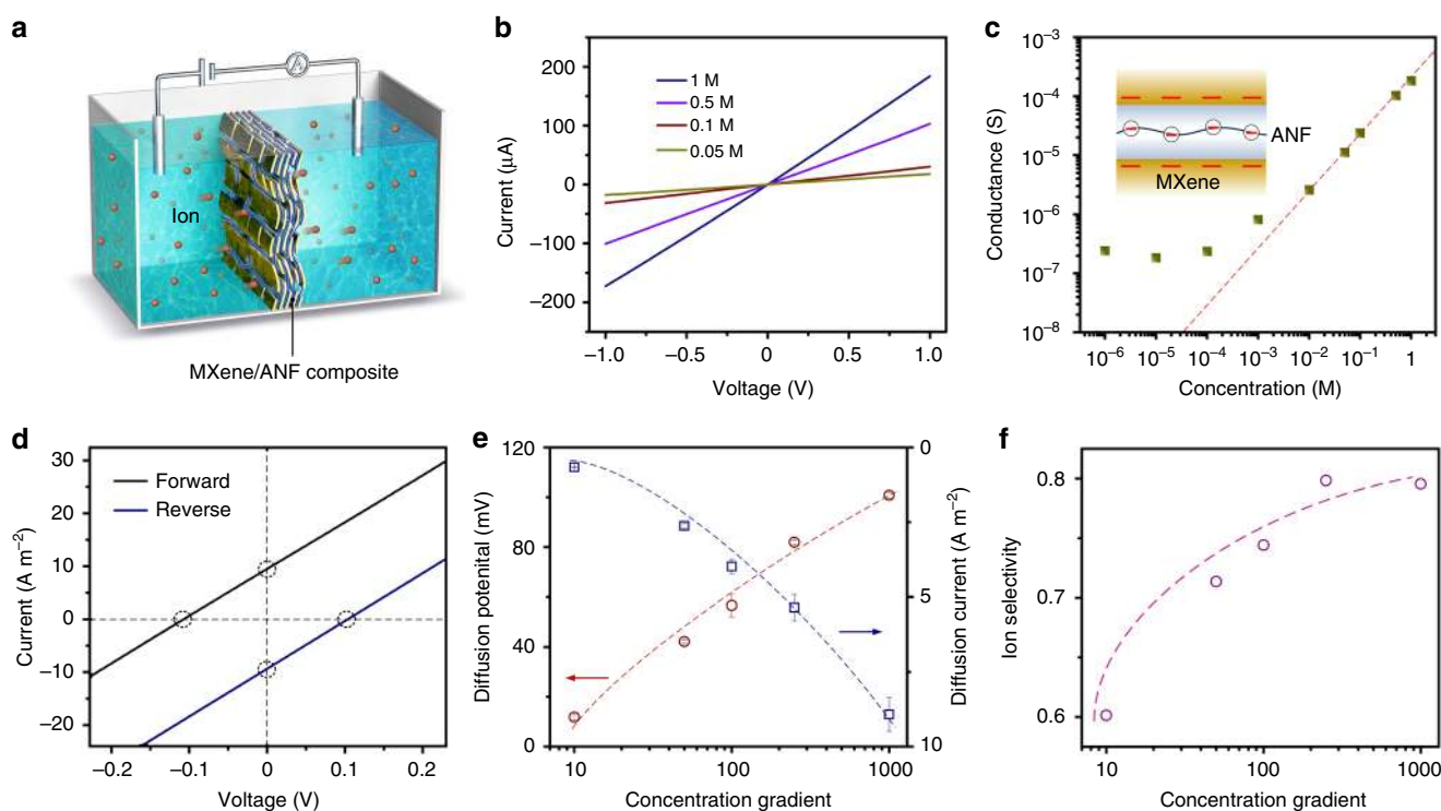
Fig. 2 Transmembrane ionic transport. a Schematic of the experimental setup to measure the transmembrane ionic transport. b I - V curves of composite membrane with an ANF weight content of 11% recorded in neutral KCl electrolyte with different concentrations. c Conductance measurement in KCl electrolyte. The ionic conductance deviates from bulk value (red line) at low concentration region, indicating a charge-governed ion transport. Inset: The charged state of MXene and ANF. d I - V curves of composite membrane with an ANF weight content of 11% recorded in 1000-fold KCl concentration gradient under forward and reverse diffusion directions. e The recorded diffusion potential and diffusion current under a series of concentration gradient. The low concentration side is set to 0.1\text{ mM} . Error bars represent s.d. f The ion selectivity, defined as transmembrane ion transference number, increases from about 0.6 to 0.8 with increasing concentration gradient
