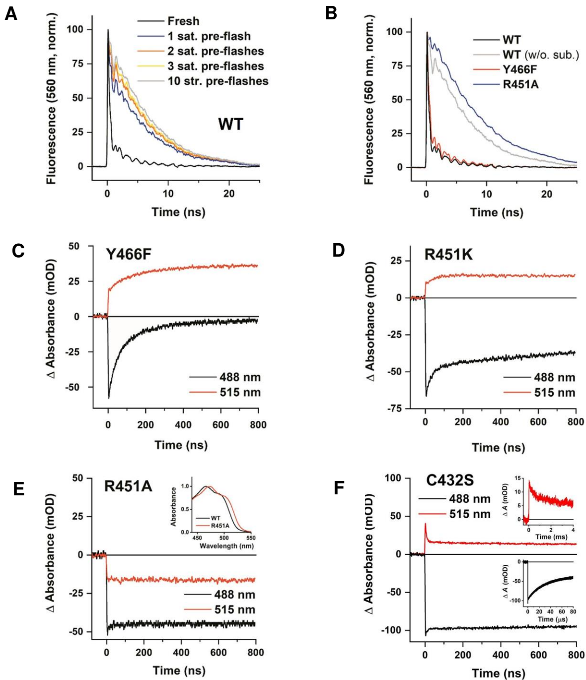
1 2 Fig. S25: Time-resolved fluorescence and transient absorption signals of WT and mutant 3 CvFAP.
