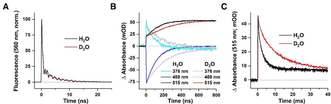
1 2 3 Fig. 3. Effects of H 2 O/D 2 O exchange on time-resolved fluorescence and UV-visible 4 spectroscopy of CvFAP. (A) Normalized signals of time-resolved fluorescence of 1 FAD* at 560 5 nm in H 2 O and D 2 O buffers. (B) Effect of H 2 O to D 2 O exchange on the kinetics of FAD •- 6 reoxidation to FAD RS followed by transient absorption spectroscopy at selected wavelengths on a 7 sub-microsecond timescale. (C) Effect of H 2 O to D 2 O buffer exchange on the decay of FAD RS 8 measured at 515 nm on the millisecond timescale.
