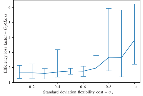
Fig. 4. Optimality loss factor OptLoss as a function of estimation inaccuracy \sigma_\lambda
