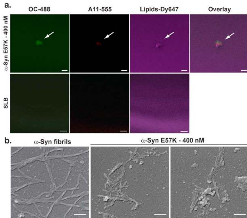
Figure 6: \alpha -Syn E57K aggregates formed on SLBs imaged by (a) immunofluorescence and (b) CryoSEM. (a) Confocal image of OC and A11 antibody bound to adsorbed \alpha -Syn E57K on donor labeled SLBs. The protein clusters formed after 24 hours of incubation were stained with the anti-amyloid antibody OC, specific to mature amyloid structures. The same particles were partially recognized by A11, an antibody specific to oligomeric amyloid precursors. SLBs without adsorbed protein were incubated with the same antibodies as a control Scale bars: 2 \mu m for the E57K sample and 20 \mu m for the control. (b) CryoSEM images of aggregates formed on SLBs after 24 hours of incubation with 400 nM E57K \alpha -Syn solution as indicated. The left panel shows a bilayer briefly incubated with \alpha -Syn fibrils aggregated in solution. The two panels to the right show two areas of \alpha -Syn E57K aggregated on SLB Scale bars: 100 nm.
