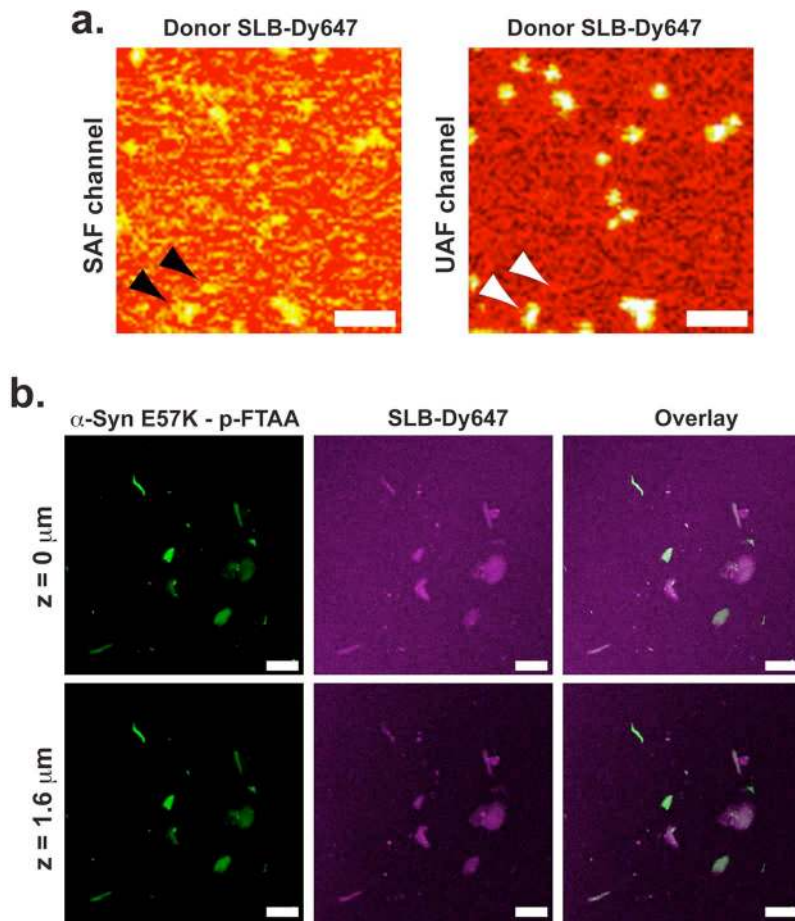
Figure 3: Fluorescent microscopy images showing lipid extraction away from the plane of the SLB. a) Addition of unlabeled A53T \alpha -syn (400 nM) to a fluorescent SLB, as most of the aggregates show more intense fluorescence in the UAF channel (top arrows) indicating lipid extraction from the SAF detection volume, bottom arrows shows an area of clustered lipids that is only present in the SAF channel therefore confined to the surface of the SLB. b) Confocal images corresponding to different z-planes of a z-stack. The p-FTAA stained E57K aggregates formed on the SLB at a starting protein concentration of 3 \mu\text{M} (left column) are surrounded by lipids (middle column, lipids labeled with Dy647). The closest plane to the bilayer is indicated as z = 0 \mu\text{m} .
