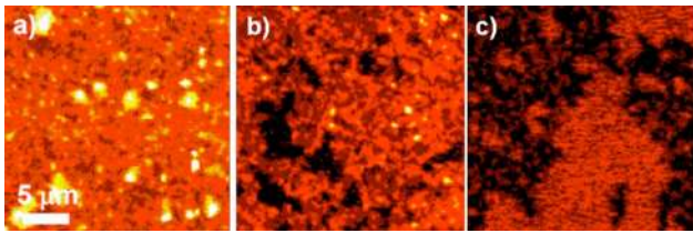
Figure 4: SAF images showing membrane damage to donor labeled SLBs by WT and E57K \alpha -Syn. (a) and (b) show SLBs 24 hours after WT protein incubation of 1.5 \mu M and 3 \mu M respectively, (c) shows SLBs 24 hours after incubation of a 1.5 \mu M solution of E57K \alpha -Syn. All images 0 – 200 au (black to yellow).
