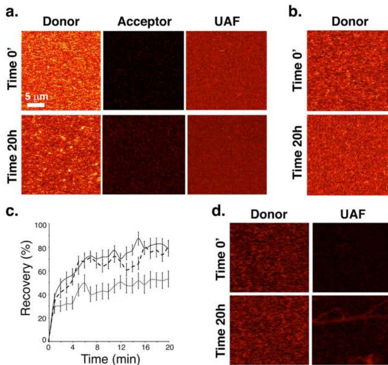
Figure 7: a) SAF and UAF images showing the adsorption of acceptor labeled 400 nM E57K \alpha -Syn onto donor labeled SLBs in the presence of 400 nM dopamine, b) SAF image of adsorption of dopamine alone on donor labeled SLB c) FRAP analysis of the lipid mobility of donor labeled SLBs alone (solid line), donor labeled SLB plus 400 nM dopamine after 20 h (large dashes), and donor labeled SLB plus 400 nM E57K \alpha -syn and 400 nM dopamine after 20 h (small dashes). d) SAF and UAF images of donor labeled SLB before and after addition of 3 \mu M unlabeled E57K pre-formed fibers. All donor and UAF scans shown on a scale of (0-200 au) and all acceptor scans (0-50 au).
