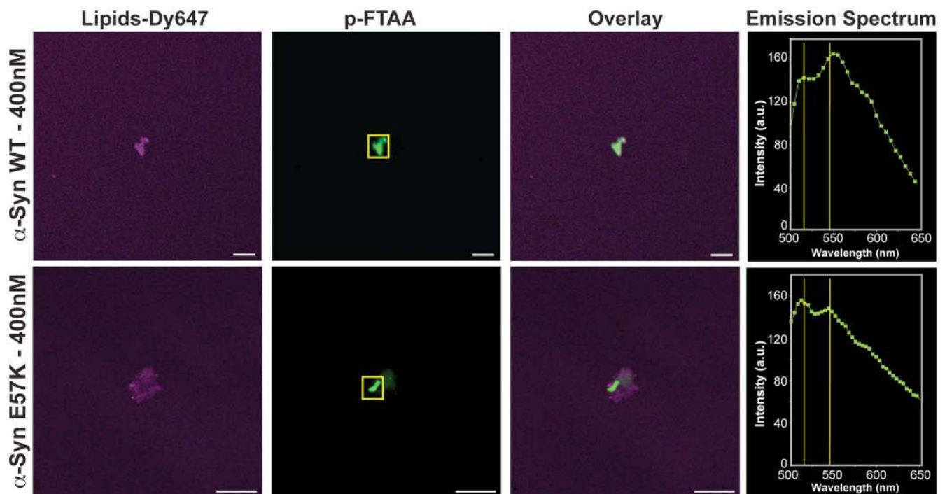
Figure 5: Characterization by confocal microscopy of \alpha -Syn aggregates formed on SLBs. Donor labeled SLBs were incubated for 24 hours with the indicated \alpha -Syn variants before addition of the p-FTAA dye. Emission spectra of fluorescent areas were acquired to confirm the presence of cross \beta -sheet rich entities. For WT \alpha -Syn the excitation wavelength was 405 nm, for \alpha -Syn E57K - 400 nm it was 488 nm. The emission spectra were taken from areas highlighted by the yellow boxes. Scale bars: 10 \mu m.
