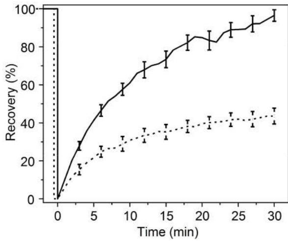
Figure 1: Lipid mobility is decreased by the presence of \alpha -Syn measured by FRAP. FRAP from donor labeled SLB before (solid line) and 24 h after adsorption and incubation of 400 nM \alpha -Syn (dashed line). Photobleaching at time 0' was achieved using a pulsed laser (635 nm) at an intensity of 1.6 mW for 10 min.
