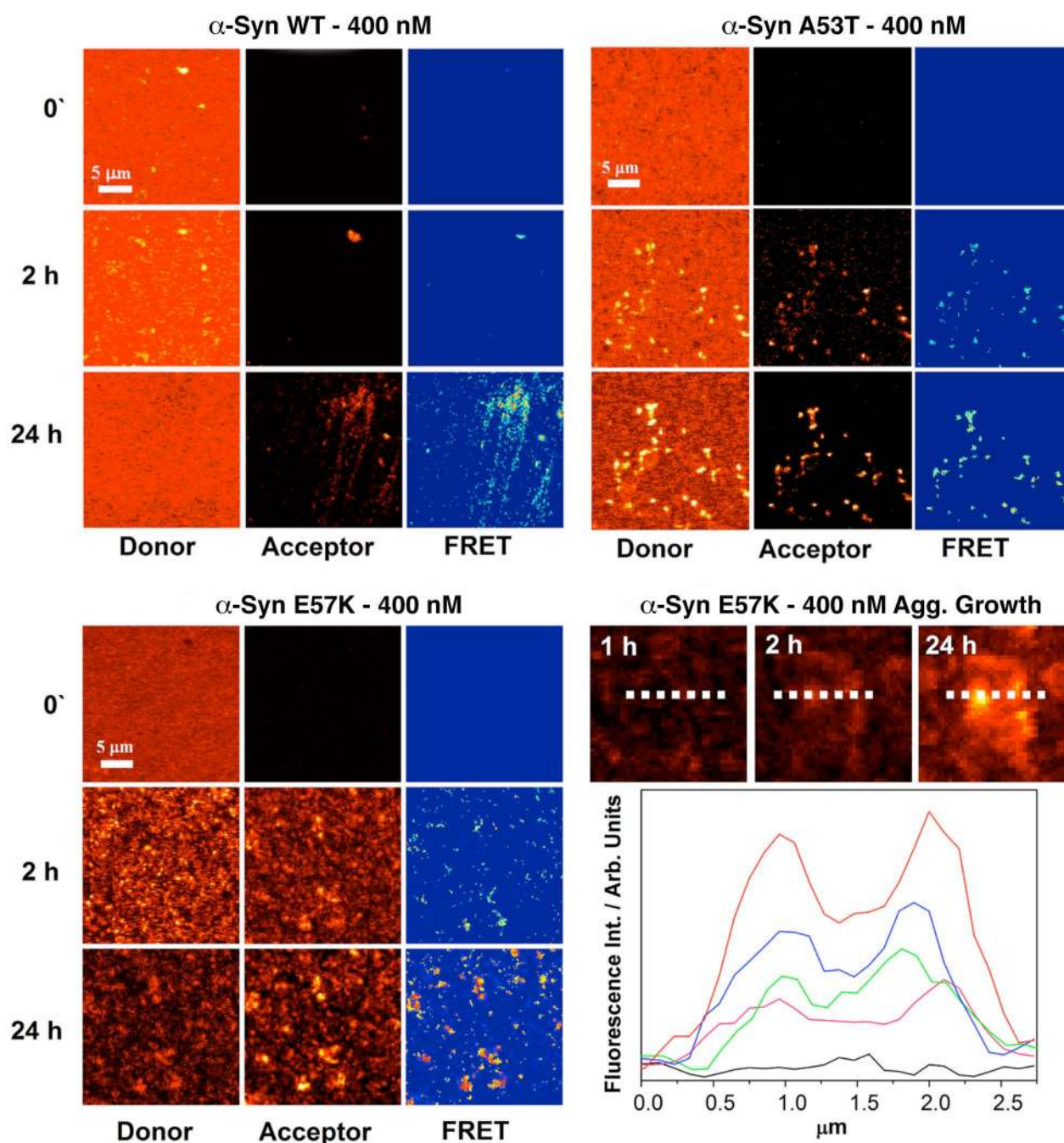
Figure 2: SAF images at different incubation times (0, 2, and 24 h) showing adsorption of 3 variants of acceptor labeled \alpha -Syn onto donor labeled SLBs. For each variant the left column shows fluorescence from the donor channel 0 – 200 (red to yellow) arbitrary units (au), the centre column fluorescence from the acceptor channel 0 – 50 au (black to red), and the right column shows FRET intensities 0 – 30% (blue to red). The fourth panel shows the evolution of the growth of one aggregate at 1 h (black line), 2 h (pink), 4 h (green), 8 h (blue), and 24 h (red) after injection of \alpha -Syn E57K.
