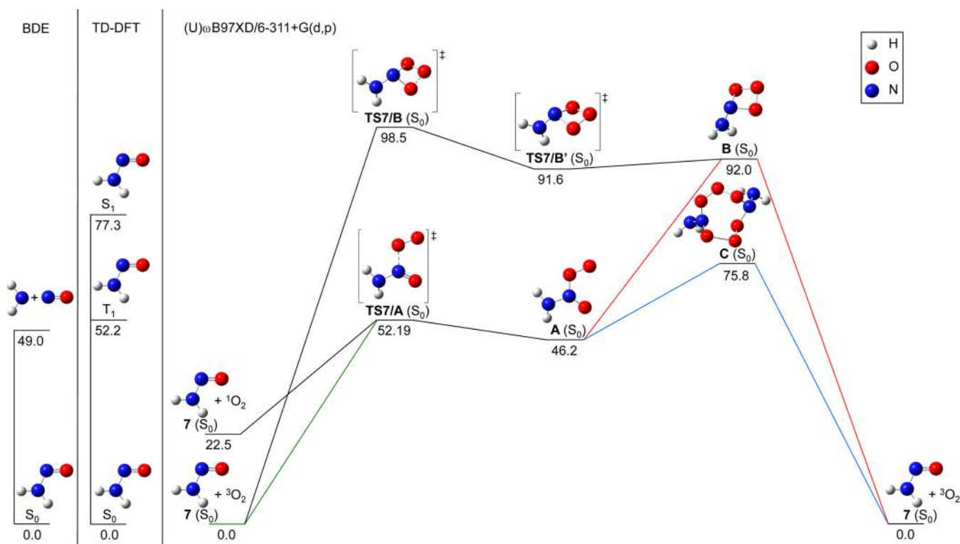
Figure 3. DFT and TD-DFT computed BDE and excited states of nitrosamine 7 . DFT potential energy surface with structures and transition states (TS) for the reaction nitrosamine 7 with triplet and singlet oxygen. The experimental value for 3 O 2 / 1 O 2 gap (22.5 kcal/mol) has been used. Energetics in kcal/mol.
