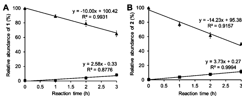
Figure 2. HPLC/MS isotopic abundances of nitrosamine reagent [(M + H)^+] ( \blacktriangle ) and ^{18}\text{O} -labeled nitrosamine product [(M + 2) + H]^+ ( \blacksquare ) as a function of photolysis time of 1 (A) and 2 (B) with ^{18}\text{O}_2 in acetonitrile. The sum of the isotopic abundance of the two peaks and [(M + 1) + H]^+ was normalized to 100%.
