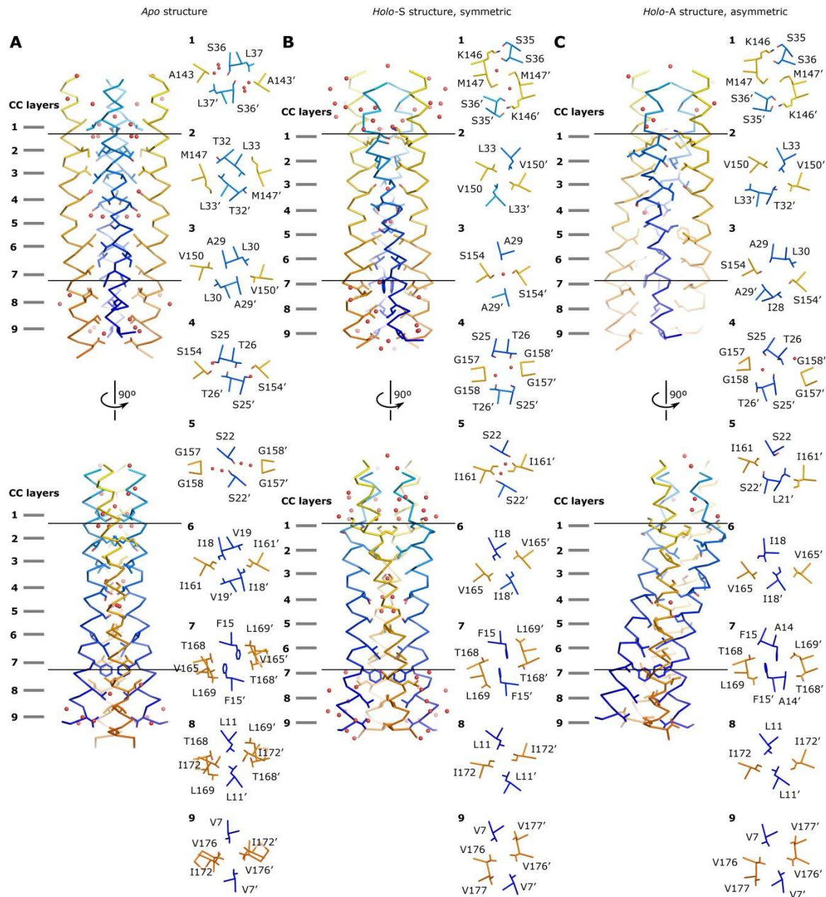
1 2 Figure S4. Structure of the NarQ transmembrane domain. TM1 is in blue, and TM2 is in yellow. (A) Apo state. 3 (B) Symmetric holo state. (C) Asymmetric holo state. In each panel, overall structure (left) and side chain packings 4 in the 9 CC layers (right, view from the periplasm) are shown. In each structure, ordered water molecules are 5 observed in or around CC layer 4. 6 7
