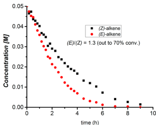
Figure 4. Competition experiment between ( Z )- and ( E )-hept-4-en-2-ol.
