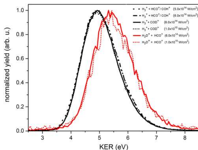
Figure 8. Kinetic energy release (KER) during the formation of trihydrogen cations at different focal intensities for dissociative ionization of CH 3 OH and CH 3 OD. All H 3 + formation channels (black curves) represent a Gaussian distribution with a mean of 5.00 eV and a standard deviation of 0.62 eV, while H 2 D + formation channels (red curves) have a similar distribution with a mean of 5.48 eV and a standard deviation of 0.69 eV.
