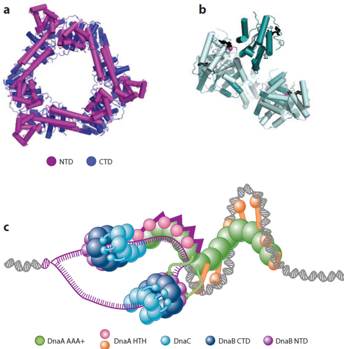
Figure 4. DnaB structure and loading. (a) Closed-ring DnaB hexamer from Bacillus stearothermophilus (128). (b) Structure of a spiral DnaC oligomer [AAA+ (ATPases associated with various cellular activities) domains] bound to nucleotide (147). (c) Model for loading of DnaB onto oriC following the two-state mechanism shown in Figure 1c (147). Abbreviations: CTD, C-terminal domain; HTH, helix-turn-helix; NTD, N-terminal domain.
