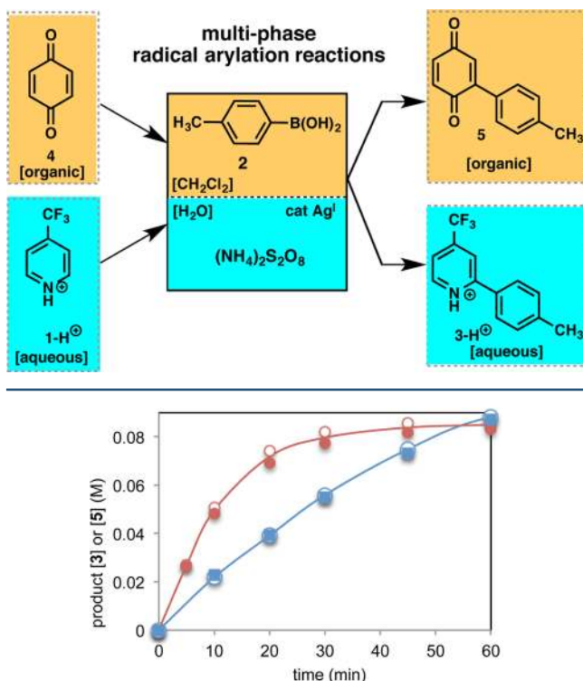
Figure 1. Effect of concentration of p -tolylboronic acid 2 on the temporal product concentration in the reactions of Scheme 1. Red symbols: CF 3 -pyridine 1 (0.1 M) to form product 3. Blue symbols: benzoquinone 4 (0.1 M) to form product 5. Solid symbols: 0.15 M p -tolylboronic acid 2. Open symbols: 0.3 M p -tolylboronic acid 2. 20 mol % Ag(NO 3 ) as catalyst, 0.3 M (NH 4 ) 2 S 2 O 8 ; CH 2 Cl 2 :H 2 O = 1:1; T = 25 °C. Reactions with 1 include 1 equiv of TFA (see Supporting Information).
