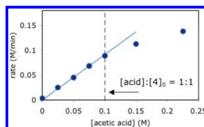
Figure 3. Effect of added acid concentration on reaction rate for the reaction in Scheme 1 with [1] = 1.2 M, [2] = 1.0 M, and [4] = 0.1 M. Rate measured from reaction calorimetric profiles at 20% conversion.
