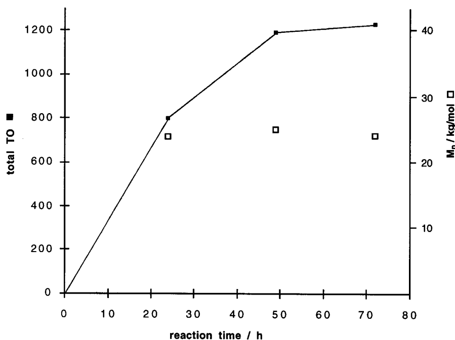
Figure 2. Reaction profile of ethylene-MA copolymerization employing ligand \text{ArN}=\text{C}(\text{Me})-\text{C}(\text{Me})=\text{NAr} ( \text{Ar} \equiv 2,6\text{-C}_6\text{H}_3(i\text{-Pr})_2 ) ( b ). Reaction conditions of entry 5, Table 2.
