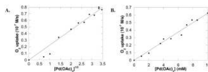
Figure 5. (A) Dependence of the initial rate on the square root of Pd(OAc) 2 concentration in the presence of large excess of pyridine. Conditions: [pyridine] = 120 mM, [amide] = 100 mM, 4.0 ml of toluene, initial pO_2 = 700 torr, 80 °C. (B) Dependence of the initial rate on the concentration of Pd(OAc) 2 in the presence of excess pyridine and acetic acid. Conditions: [pyridine] = 120 mM, [AcOH] = 5 mM, [amide] = 100 mM, 4.0 ml of toluene, initial pO_2 = 700 torr, 80 °C.
