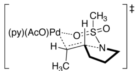
six-membered TS \Delta G^\ddagger > 35 \text{ kcal/mol}
