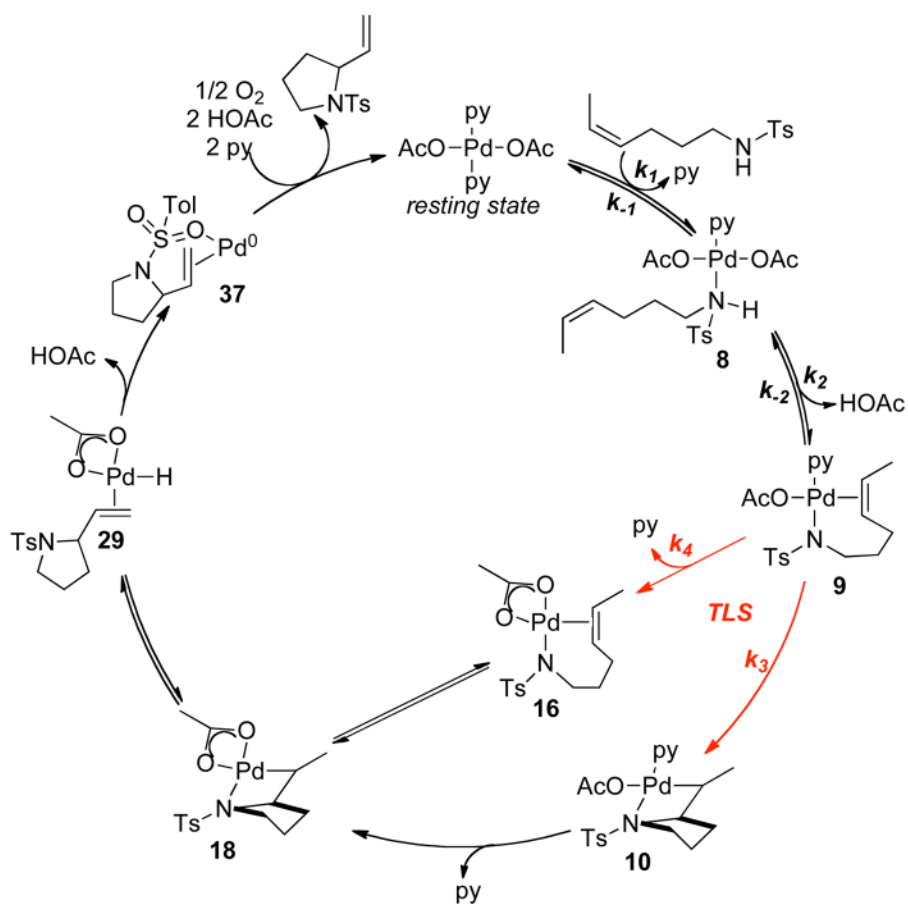
Scheme 7. Refined Catalytic Mechanism for \text{Pd}(\text{OAc})_2 /Pyridine-Catalyzed Aerobic Oxidative Intramolecular Amination of Alkenes.
