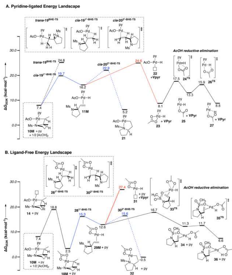
Figure 11. Low-energy pathways for the \beta -hydride elimination and AcOH-reductive-elimination. All reactions are relative to (\text{py})_2\text{Pd}(\text{OAc})_2 + \mathbf{1M} ; free py and \frac{1}{2}[\text{AcOH}]_2 . (A) Pyridine-ligated pathway; (B) Pyridine-dissociated pathway.
