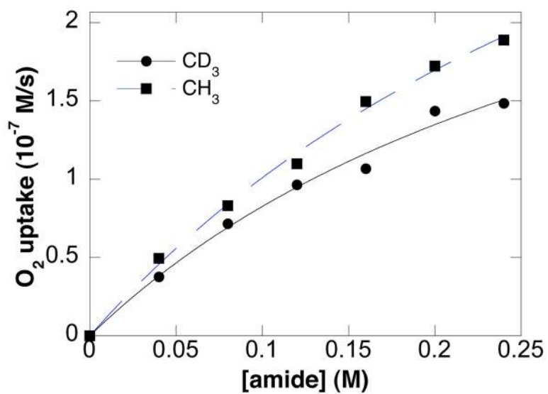
Figure 7. Dependence of the initial O 2 uptake rate on amide concentration. CH 3 - vs. CD 3 -labelled tosylamides. Conditions: [Pd(OAc) 2 ] = 2.0 mM, [pyridine] = 8.0 mM, [amide] = 0–240 mM, 4.0 ml of toluene, initial pO_2 = 700 torr, 80 °C.
