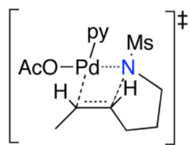
iso-13 AP -TS \Delta G^\ddagger = 24.3 \text{ kcal/mol}
