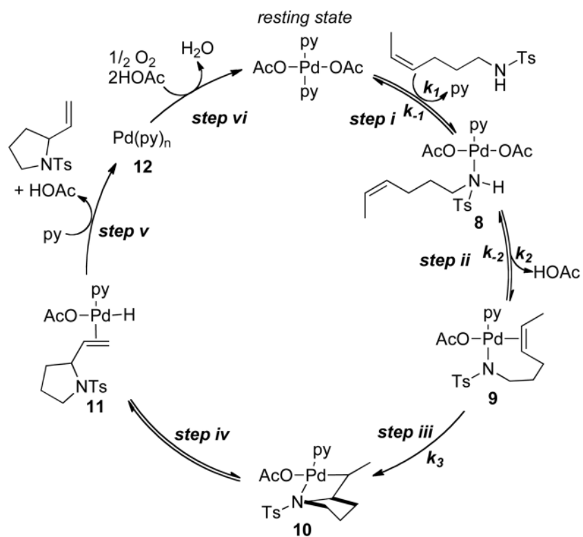
Scheme 5. Proposed Catalytic Mechanism for \text{Pd}(\text{OAc})_2/\text{Pyridine} -Catalyzed Aerobic Oxidative Intramolecular Amination of Alkenes.
