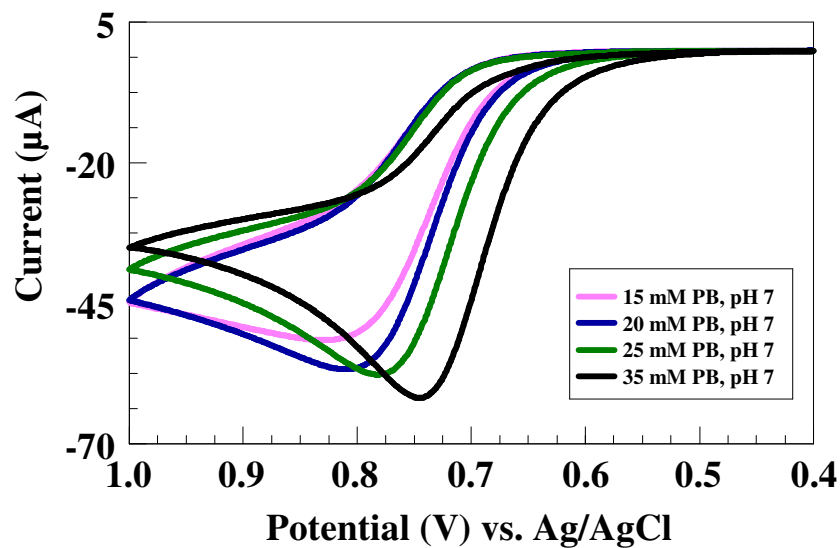
Figure 37. Plot of i ( \mu\text{A} ) vs. E (V) of the oxidation of homocysteine (3.0 mM) by \text{IrCl}_6^{2-} (1.0 mM) in various concentrations of sodium phosphate buffer containing 0.1 M NaCl at pH 7.0. Pink (15 mM PB), Blue (20 mM PB), Green (25 mM PB), and Black (35 mM PB). Scan rate: 100 mV/s.
