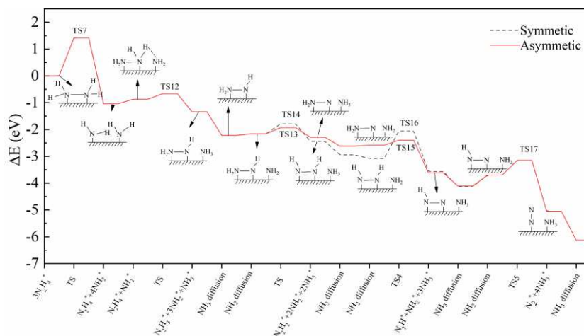
Figure 14 . Intermolecular dehydrogenation of hydrazine via \text{NH}_2 attack pathways over the Ir(111) surface. TS indicates the energy of the transition energies.
