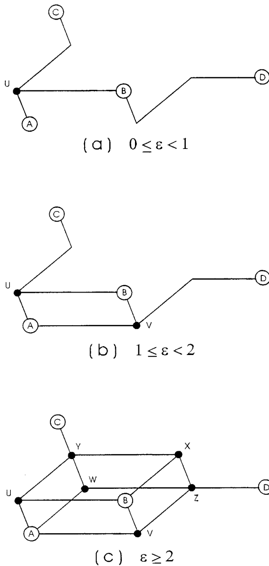
FIG. 4.—MJ networks (drawn to scale) constructed from the data of table 1 with three different settings (a–c) of the parameter \varepsilon ; inferred sequence types U , V , W , X , Y , and Z are added to the growing network as median vectors.
