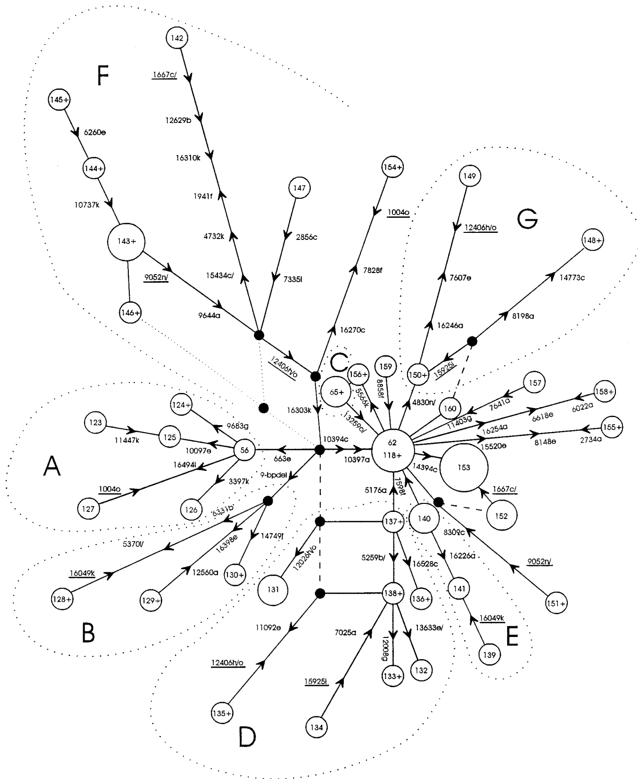
FIG. 6.—MJ network ( \epsilon = 0 ) for Tibetans, based on mtDNA restriction sites (Torroni et al. 1994; sites 10394 Dde I and 10397 Alu I are weighted 1/2; site 16517 Hae III is disregarded, but its presence is indicated by “+” accompanying the sequence types; an error in the original table concerning the status of 10394 Dde I/10397 Alu I in mtDNA type 118 has been corrected). Designation of sequence types, restriction sites, and mtDNA groups A to G accords with Torroni et al (1994). A slash indicates that a site is recognized by more than one restriction enzyme, and underlining denotes resolved recurrent mutations. Arrows point to presence of restriction sites; areas of circles are proportional to the numbers of sampled individuals. The dotted links do not appear in any MP trees; the unbroken links indicate a plausible MP tree (see text).
