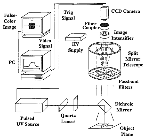
Fig. 1. Setup of the multicolor fluorescence imaging system.
