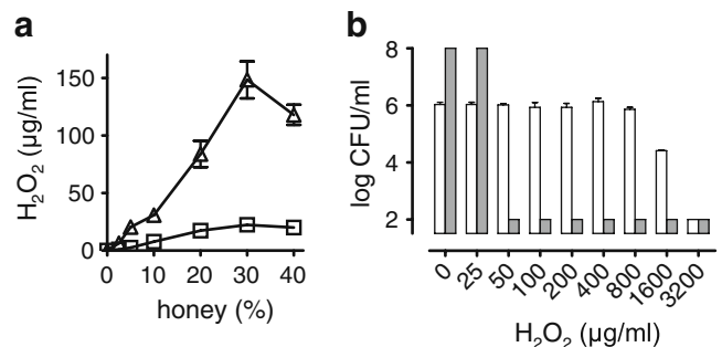
Fig. 3a, b Concentration of \text{H}_2\text{O}_2 required for activity against MRSA. a Production of \text{H}_2\text{O}_2 in diluted RS honey. The accumulation of \text{H}_2\text{O}_2 in indicated concentrations of RS honey was assessed at 2 h (squares) or 24 h (triangles) after dilution. b Bactericidal activity of solutions containing only \text{H}_2\text{O}_2 . The survival of MRSA was assessed after 2 h (white bars) or 24 h (gray bars) of incubation with the indicated concentrations of \text{H}_2\text{O}_2
