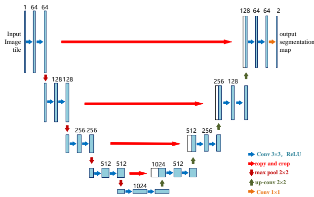
Fig. 3. The U-Net architecture [7].
