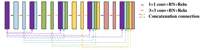
Fig. 6. Dense connection architecture [70].
