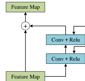
Fig. 5. The recurrent residual convolutional unit from 2018 recurrent.
