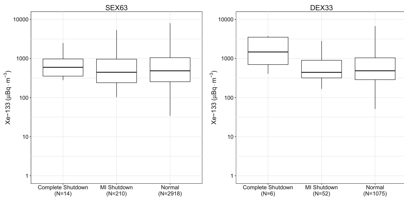
Fig. 4 Observations at the European CTBT sites located in Stockholm, Sweden (SEX63) and Schausland, Germany (DEX33). The number of samples, N , for each box plot is shown in the label
