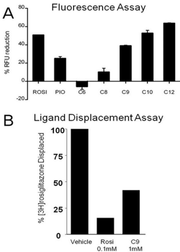
Figure 2. C8–C10 MCFAs bind and stabilize PPAR \gamma LBD in vitro .
