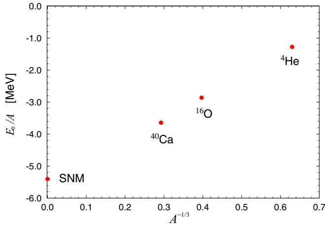
FIG. 5. (Color online) Mass number A dependence of nuclear energy per nucleon E_0/A for M_{\text{PS}} \simeq 470 MeV. The Bethe-Weizsäcker mass formula up to the second term, E_0/A = -a_V - a_S A^{-1/3} , corresponds to a straight line in this figure.
