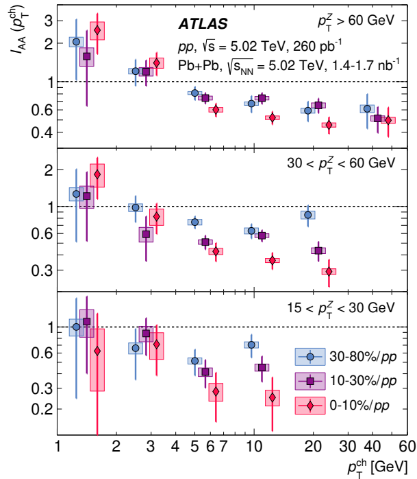
Figure 2: Ratio of the charged-particle yield in Pb+Pb collisions to that in pp collisions, I_{AA} , as a function of charged-particle p_T^{\text{ch}} , for the selection \Delta\phi > 3\pi/4 . The vertical bars and boxes correspond to the statistical and systematic uncertainties of the data. The 0–10% and 30–80% data are offset horizontally for visibility.
