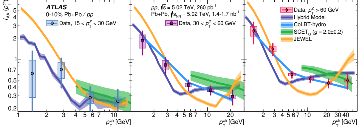
Figure 3: The I_{AA} ratio as a function of p_T^{\text{ch}} in data compared with theoretical calculations (see text), for the selection \Delta\phi > 3\pi/4 . The vertical bars and boxes correspond to the statistical and systematic uncertainties, while the shaded bands represent the theoretical uncertainty (statistical for JEWEL, Hybrid, and CoLBT-hydro, parametric for SCET _G ). The I_{AA} is shown for 0–10% Pb+Pb events for p_T^Z = 15 –30 GeV (left), 30–60 GeV (center) and > 60 GeV (right).
