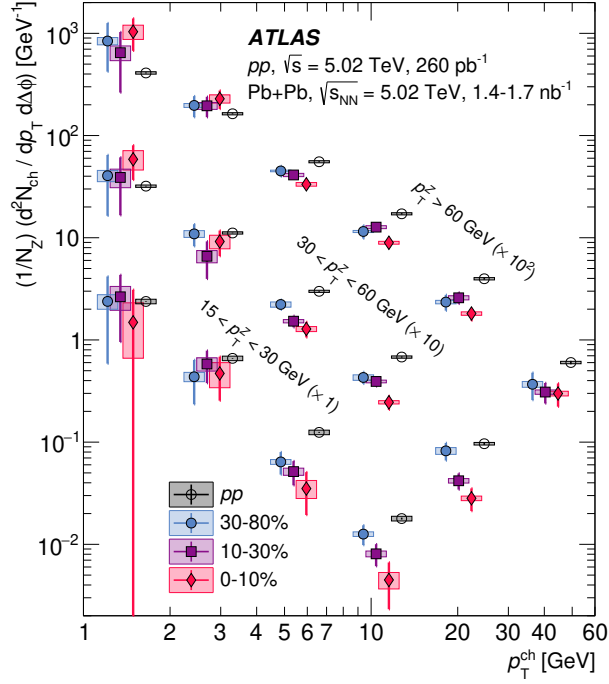
Figure 1: Charged-particle yield per Z boson as a function of p_T^{\text{ch}} , for the selection \Delta\phi > 3\pi/4 , reported for 15 < p_T^Z < 30 \text{ GeV} , 30 < p_T^Z < 60 \text{ GeV} , and p_T^Z > 60 \text{ GeV} . Results are shown for pp events and the three centralities of Pb+Pb events. These are offset horizontally around the bin centers, which are located between the 0–10% and 10–30% points, for visibility. The vertical bars and boxes correspond to the statistical and systematic uncertainties of the data.
