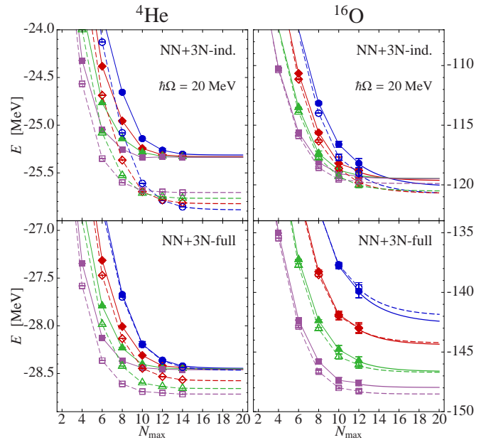
FIG. 1: (color online) IT-NCSM ground-state energies for {}^4\text{He} and {}^{16}\text{O} as function of N_{\text{max}} for the NN+3N-induced and the NN+3N-full Hamiltonians for a range of flow parameters: \alpha = 0.04 \text{ fm}^4 ( \bullet ), 0.05 \text{ fm}^4 ( \blacklozenge ), 0.0625 \text{ fm}^4 ( \blacktriangle ), 0.08 \text{ fm}^4 ( \blacksquare ). Solid symbols correspond to the exact 3N interaction, open symbols to the NO2B approximation. Error bars indicate the uncertainties of the threshold extrapolations of the IT-NCSM. Data points are connected by straight lines to guide the eye, beyond the largest N_{\text{max}} an exponential extrapolation fitted to the last four data points is shown.
