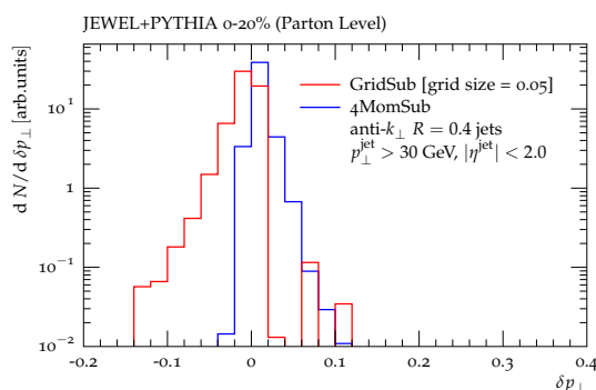
Figure 5. Relative p_{\perp} difference \delta p_{\perp} = (p_{\perp}^{\text{w/o rec}} - p_{\perp}^{\text{w rec}}) / (p_{\perp}^{\text{w/o rec}} + p_{\perp}^{\text{w rec}}) between parton level jets reconstructed with and without recoiling partons for the two subtraction methods.
