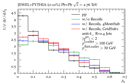
Figure 8. Di-jet momentum asymmetry A_J = (p_{\perp}^{\text{LeadJet}} - p_{\perp}^{\text{SubLeadJet}})/(p_{\perp}^{\text{LeadJet}} + p_{\perp}^{\text{SubLeadJet}}) for central Pb+Pb central events in JEWEL+PYTHIA. The green line represents JEWEL+PYTHIA without medium response while the blue and red lines show the result including medium response with 4MomSub and GridSub1 respectively.
