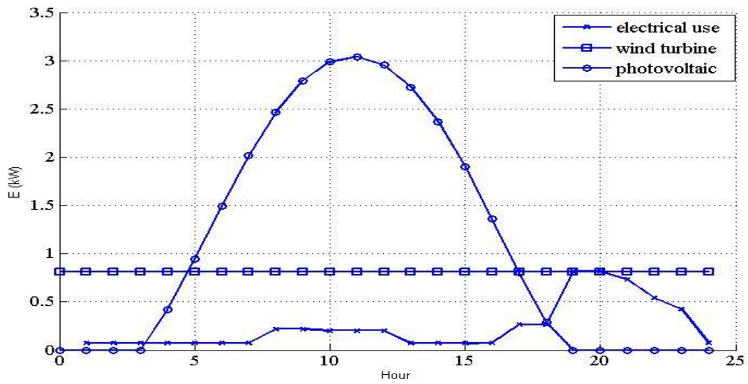
Fig.6. Electrical output of the PV, wind turbine and battery, and electrical usage, on July15
