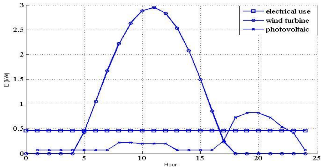
Fig.7. Electrical output of the PV, wind turbine and battery, and electrical usage, on January 15
