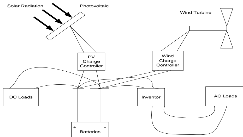
Fig. 3. General diagram of a hybrid (wind-PV) system [2]
