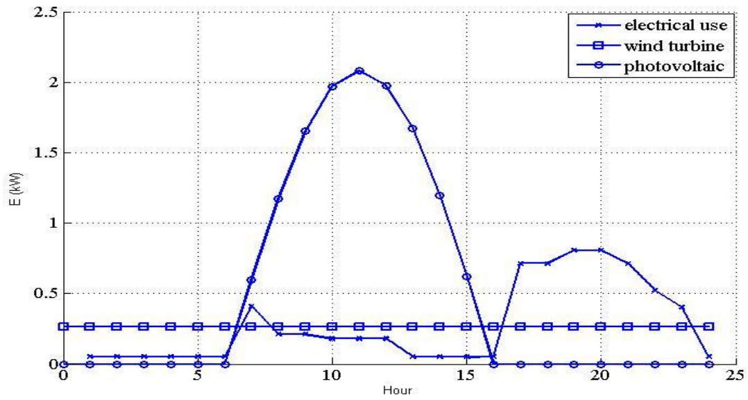
Fig.5. Electrical output of the PV, wind turbine and battery, and electrical usage, on January15
