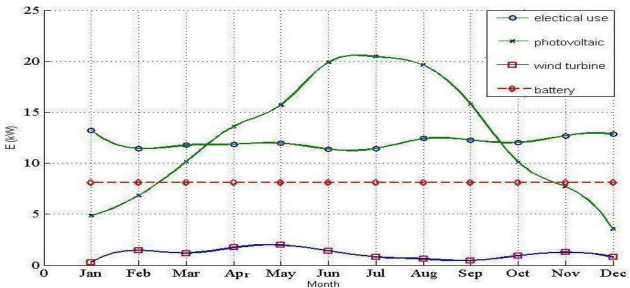
Fig.4. Annual electrical production of the system (PV, wind turbine, battery) and usage
