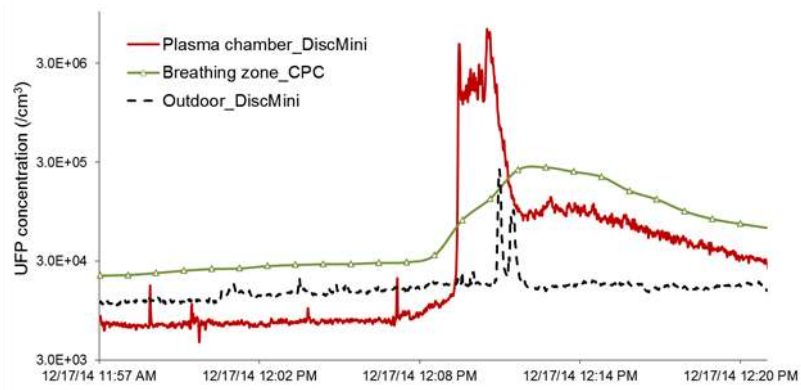
Figure 1. Ultrafine particle (UFP, 10-700 nm) concentrations monitored at three locations in a real-world industrial setting.
