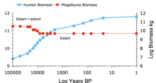
Fig. 3. Estimated biomass of humans plotted against the estimated biomass of non-human megafauna. See Methods for parameters used.
