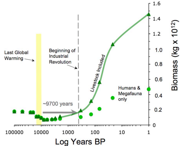
Fig. 5. Semilog plot of the sum of human and non-human wild megafauna biomass (dots) and the sum of human, wild, and domestic megafauna (triangles connected by line). Yellow bar indicates the timing of the YD-Holocene climatic event that led into the current interglacial. See Methods for parameters used.
