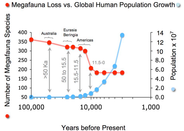
Fig. 2. Number of non-human megafauna species that went extinct through time plotted against estimated population growth of humans.
