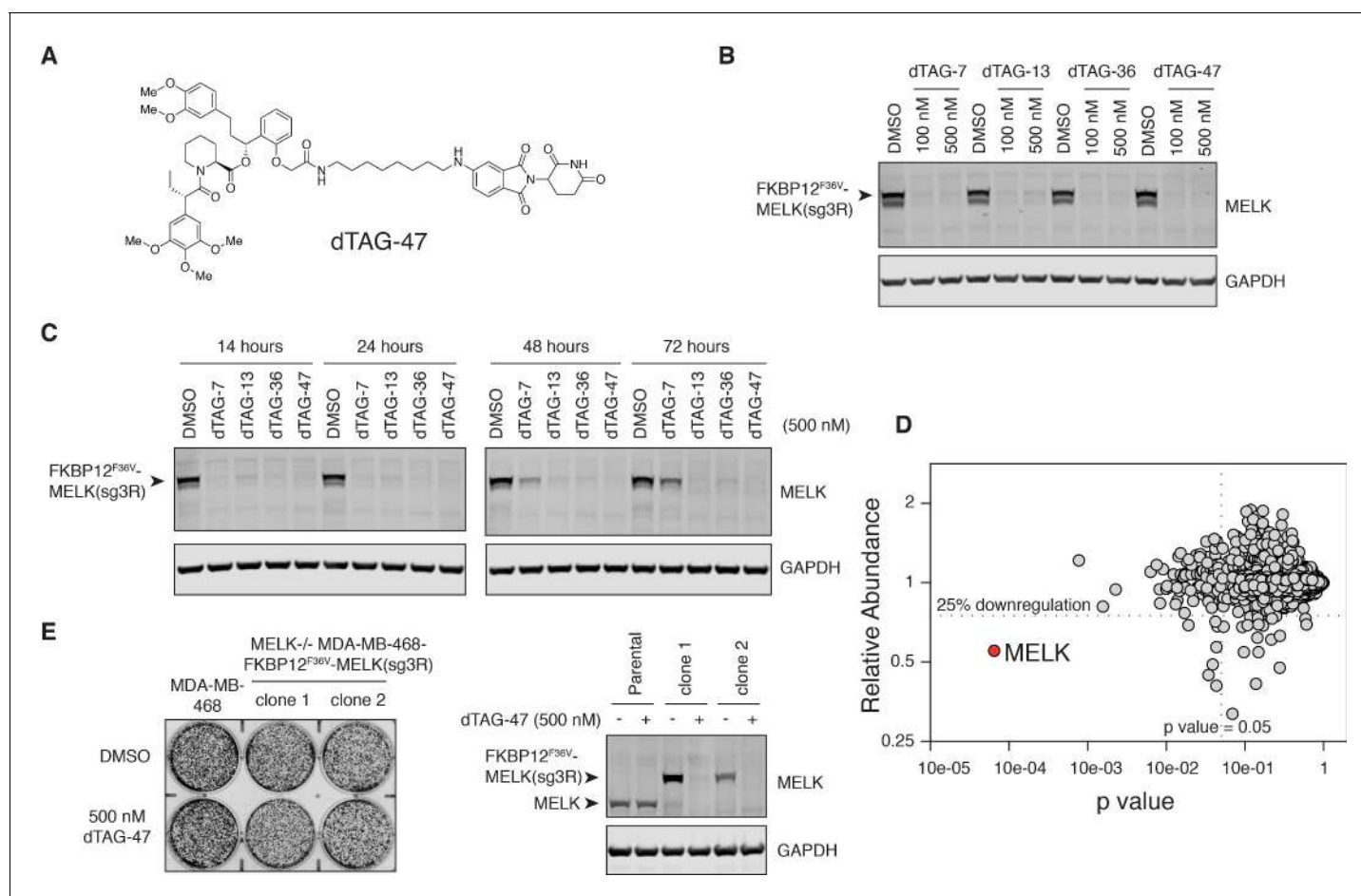
Figure 4. MELK -/- MDA-MB-468-FKBP12 F36V -MELK(sg3R) cells grow normally in response to pharmacologically induced FKBP12 F36V -MELK degradation. (A) Chemical structure of heterobifunctional dTAG molecule dTAG-47. See also Figure 4—figure supplement 3 for the chemical structures of dTAG-7, dTAG-13 and dTAG-36. (B) Immunoblots for MELK and GAPDH after treatment of dTAG-7, 13, 36, and 47 at indicated concentrations in MELK -/- MDA-MB-468-FKBP12 F36V -MELK(sg3R) cells for 4 hours. See Figure 4—figure supplement 1 for details of the generation of MELK -/- MDA-MB-468-FKBP12 F36V -MELK(sg3R) clones. (C) Same as in 4B, but with treatment at 500 nM and extended treatment times for 14, 24, 48, and 72 hours. (D) Changes in abundance of 7270 proteins (peptide count \geq 2 ) comparing MELK -/- MDA-MB-468-FKBP12 F36V -MELK cells treated with dTAG-7 (250 nM) or DMSO for 1 hour, versus p-value (dTAG-7: triplicate, DMSO: duplicate, limma moderated t-test). See also Figure 4—source data 1 and 2 for the original and the processed data. (E) Crystal violet staining image showing parental MDA-MB-468 cells and MELK -/- MDA-MB-468-FKBP12 F36V -MELK(sg3R) cells after treatment with DMSO or 500 nM of dTAG-47 for 9 days. Immunoblots showing MELK and GAPDH from a duplicate plate on Day 9 confirmed sustained depletion of FKBP12 F36V -MELK(sg3R). These are representative data from one of two independent experiments.
