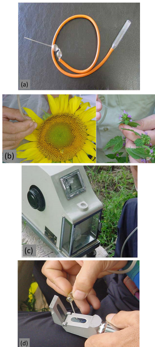
Fig. 2. Illustration of the nectar collection with the capillary pipet of the ICDA: general view of the device (a), nectar aspiration on Helianthus annuus and Lamium purpureum (b), field balance (c), refractometer (d)
