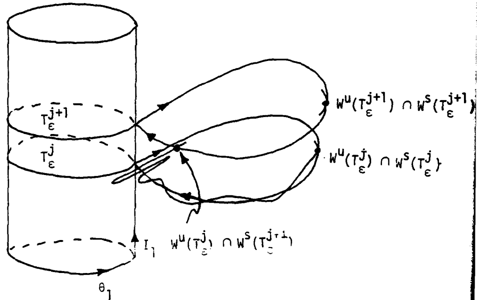
Figure 3. Intersections of manifolds and Arnold diffusion in a three degree of freedom system. The Poincaré section \theta_2 = \frac{0}{2} is shown on the energy surface H^E = h .
