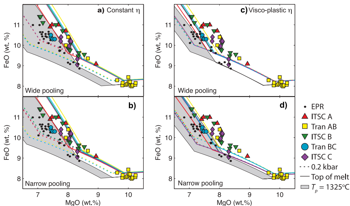
Figure 12. Liquid lines of descent (LLD) model calculations of FeO versus MgO. Colored LLD in each plot correspond to the color of the data point for each ITSC or transform fault strand as shown in the legend on the bottom right and in Figure 10. Solid LLD lines indicate fractional crystallization at the top of the melt surface, which ranges in depth from 18 to 24 km (6–8 kbar) for constant viscosity and 9–15.5 km (3–5 kbar) for viscoplastic rheology, while dashed LLD lines indicate fractional crystallization at 0.2 kbar, which would be expected for fractional crystallization in a shallow magma lens. All models were run for T_p = 1350^\circ\text{C} and Nu = 4 . The gray shaded regions indicate the predicted model region for T_p = 1325^\circ\text{C} . Models were run for (a and b) constant viscosity and (c and d) viscoplastic rheology and for a wide melt pooling region (Figures 12a and 12c) and a narrow melt pooling region (Figures 12b and 12d).
