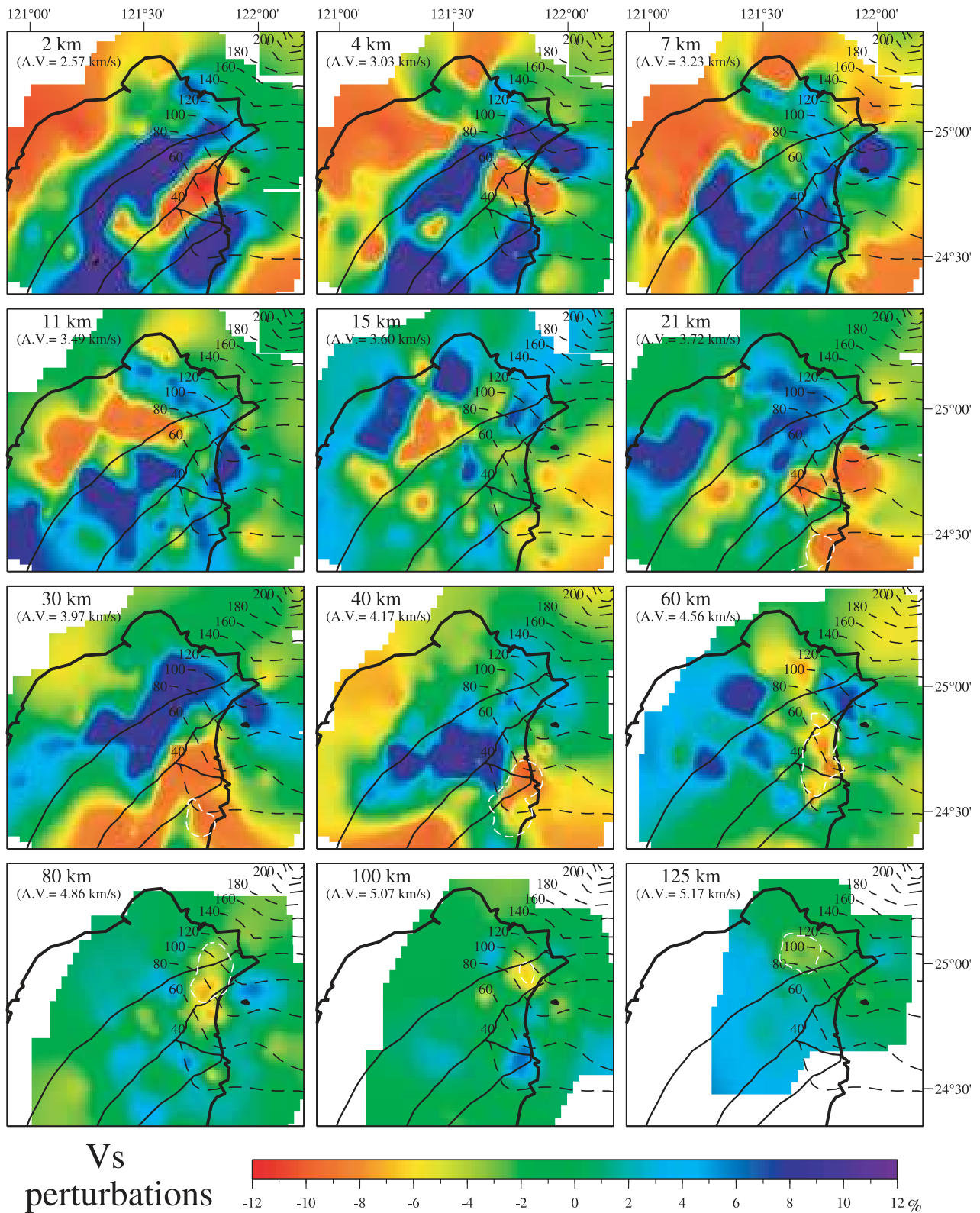
Figure 5. V_s tomography results displayed for 12 horizontal slices from 2 to 125 km. V_s values are in percentages with respect to the average S wave velocity at the depth of the slice. Legends are as in Figure 4.
