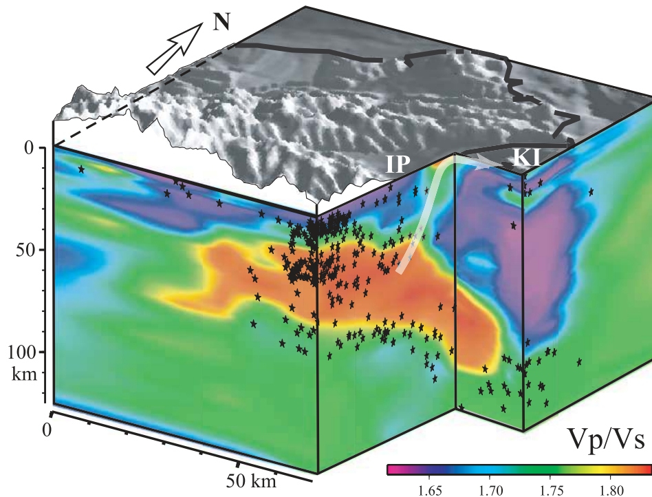
Figure 10. A 3-D block diagram showing cross sections of V_p/V_s ratios. The high V_p/V_s sausage-like body is cut along its axis (corresponding to profile 2 located in Figure 8). A high V_p/V_s channel rises obliquely (white arrow) from the sausage-like body from a depth of 40 km in direction of the andesitic Kueishantao Island (KI). IP, Ilan Plain. Stars are earthquake locations. Shaded 3-D topography is extracted from Liu et al. [1998].
