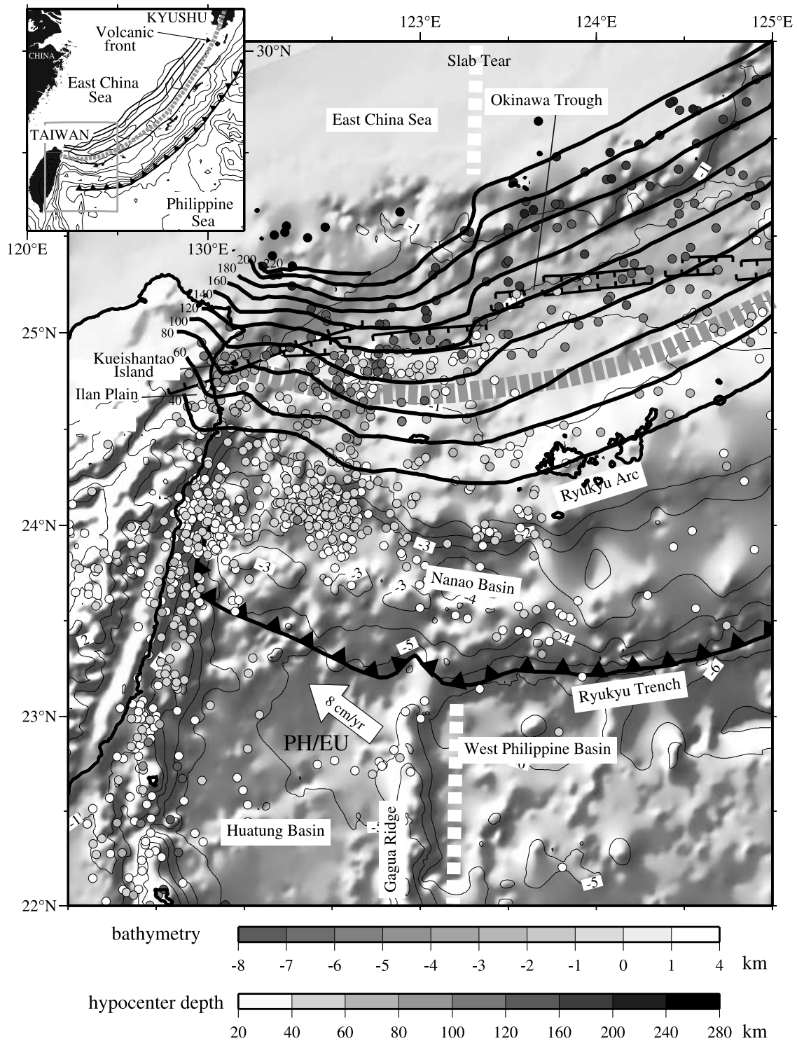
Figure 1. Shaded bathymetry and seismicity [Engdahl et al. , 1998] in the northwestern corner of the Philippine Sea plate. Dots represent earthquake hypocenters. The black contour lines are depths of the Wadati-Benioff zone (adapted from Font et al. [1999] in the western part). Inset is a general map of the Ryukyu subduction zone with slab isobaths every 50 km [Sibuet et al. , 1998]. The volcanic front (dashed gray line) is located 80–100 km above the slab. The locations of Ryukyu trench and Okinawa Trough normal faults are from Sibuet and Hsu [2004]. The arrow indicates the PH plate motion relative to EU [Yu et al. , 1997].
