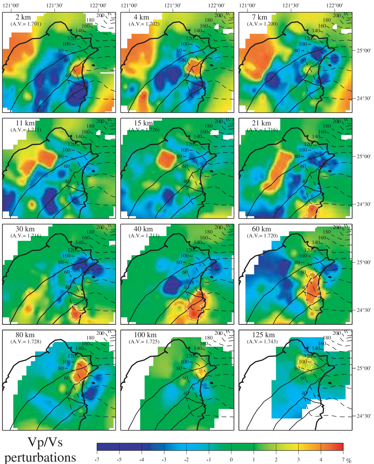
Figure 6. V_p/V_s tomography results displayed for 12 horizontal slices from 2 to 125 km. Legends as in Figure 4. The white dashed lines represent the location of V_p/V_s anomalies larger than 1.78, showing that the sausage-like body is properly imaged at depths larger than 21 km.
