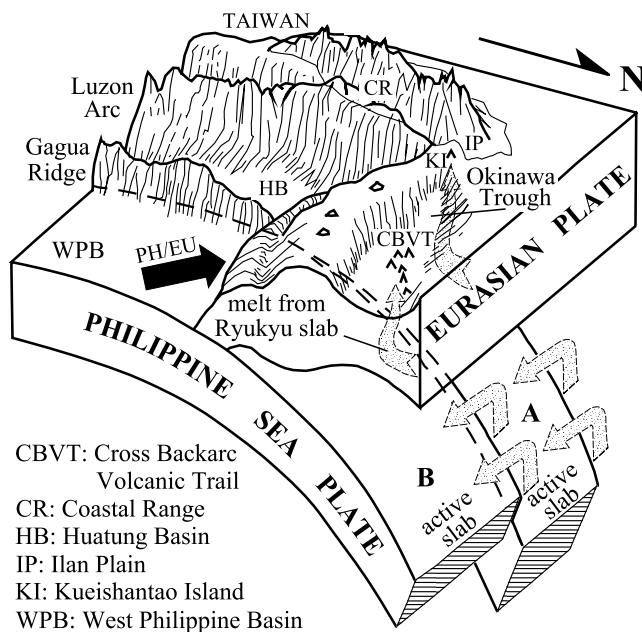
Figure 11. Diagram showing the slab tear occurring along the northern prolongation of Gagua Ridge, in the north-western corner of the Philippine Sea plate. Stippled arrows indicate fluid-migrating pathways around the slab edges (between A and B and East of A). Contorted stippled arrows give an indication of the oblique fluid and melt pathways to the cross-back-arc volcanic trail (CBVT) and Kueishantao Island. The arrow shows the direction of the Philippine Sea plate motion relative to the Eurasian plate [Yu et al. , 1997].
