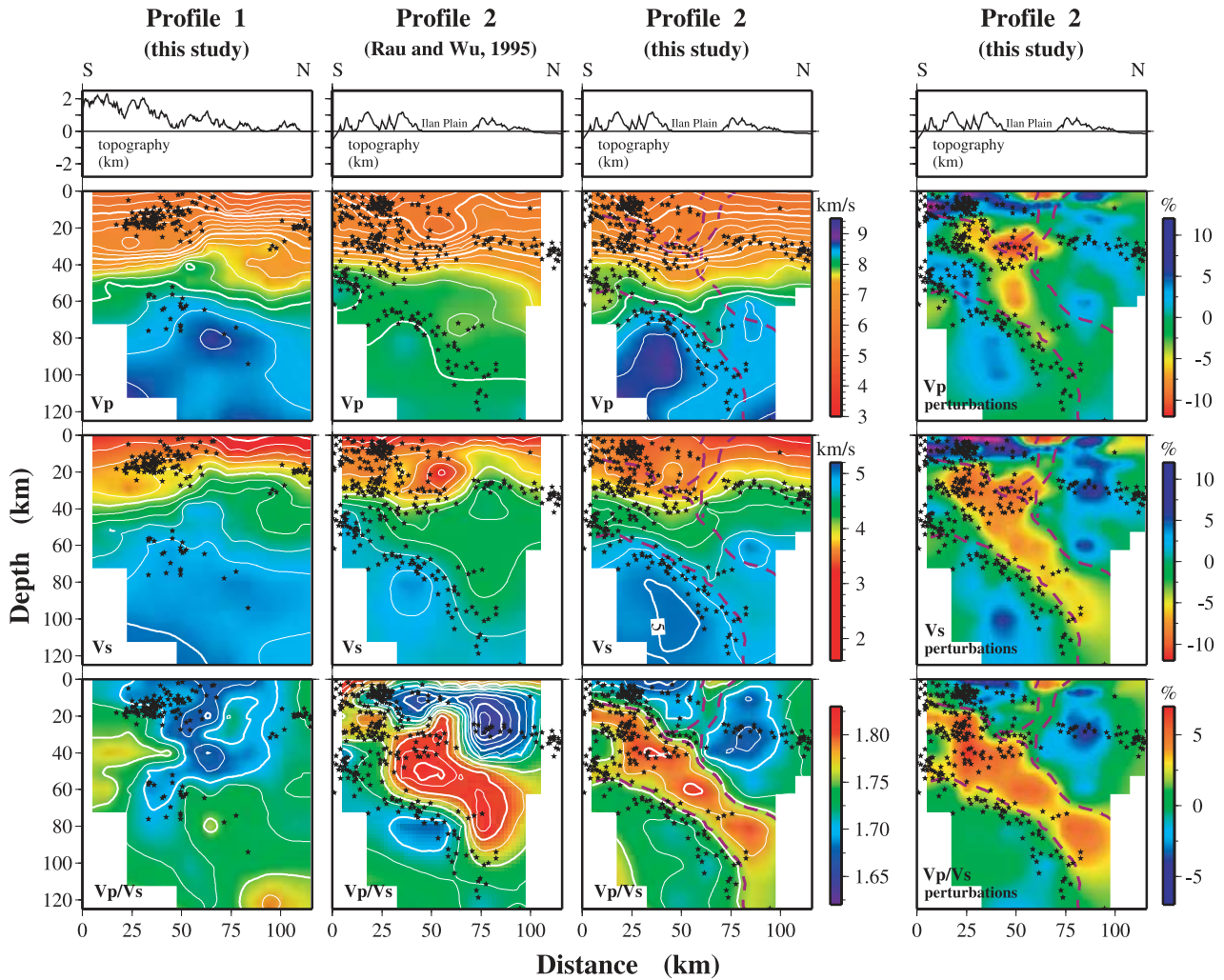
Figure 9. Tomographic results along profiles 1 and 2 located in Figure 8. (left) V_p , V_s and V_p/V_s values for profiles 1 and 2. Contours every 0.2 km/s for V_p and V_s and every 0.025 for the V_p/V_s ratio. Stars are locations of earthquakes ( M > 2.5 ) occurring in a 10 km wide stripe. Profile 1 is located on the EU continental crust, west of the Ryukyu slab edge. The few earthquakes located at depths of 50 to 80 km belong to the eastern part of the 10 km wide stripe. A comparison between results of Rau and Wu's [1995] model and ours shows the better resolution of our model and the good correspondence between the top of the Ryukyu slab and tomographic gradients. (right) V_p , V_s and V_p/V_s perturbation anomalies displayed along profile 2 in order to better image velocity anomalies of the sausage-like body and the feeding channel of Kueishantao Island. The high V_p/V_s sausage-like body and channel are underlined by red dashed lines and then pasted in the other panels.
