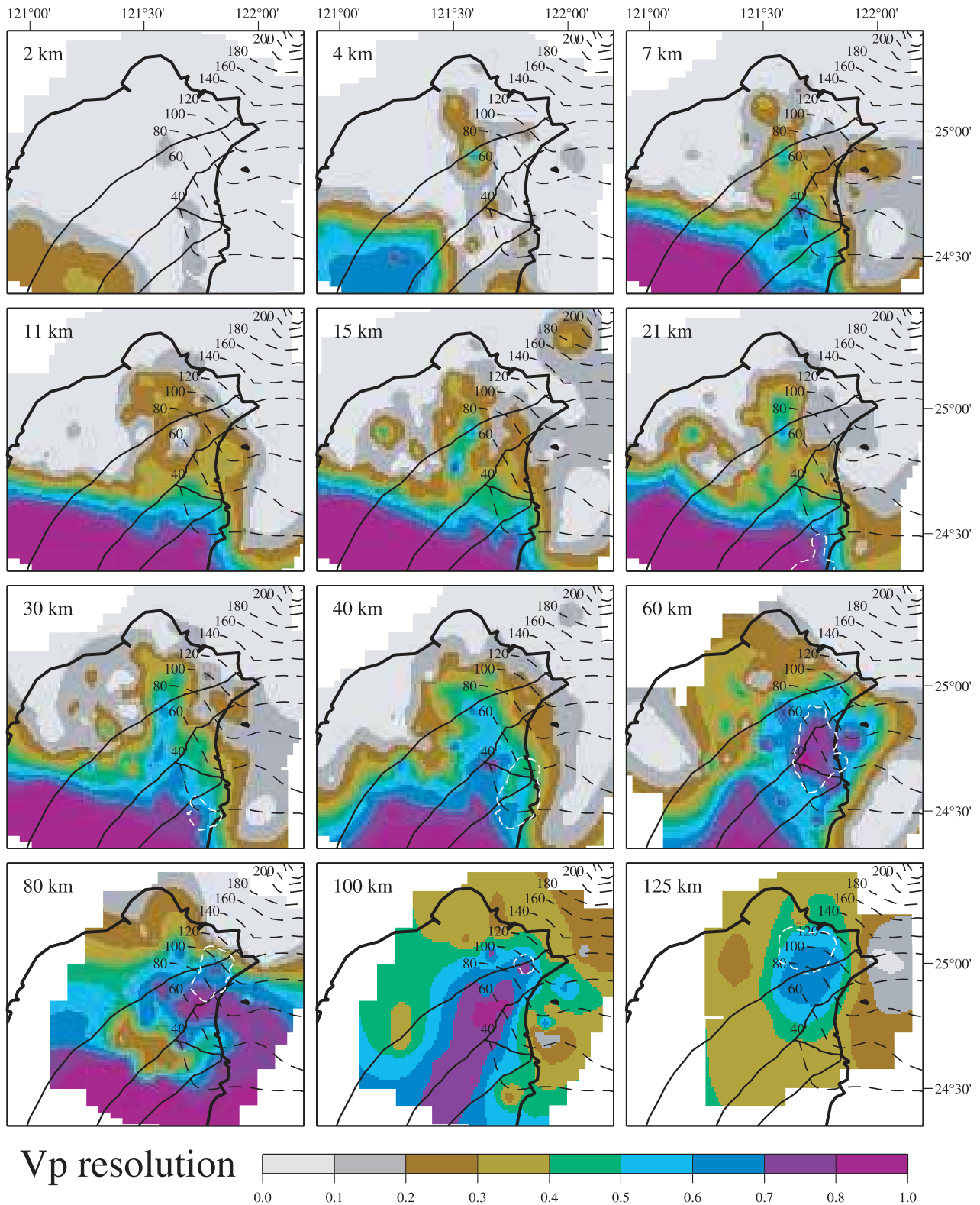
Figure 7. V_p resolution (diagonal elements of the resolution matrix) displayed for 12 horizontal slices from 2 to 125 km. Legends are as in Figure 4.
