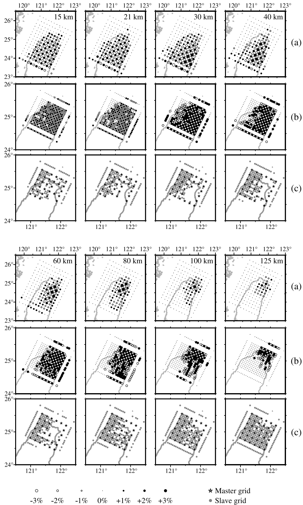
Figure 3. Results of checkerboard test resolution displayed for eight horizontal slices ranging from depths of 15 to 125 km. (a) Gridding space of 18 km; (b) gridding space of 6 km; and (c) flexible gridding method applied in areas of poor checkerboard distribution. Slave and master grids are linked.
