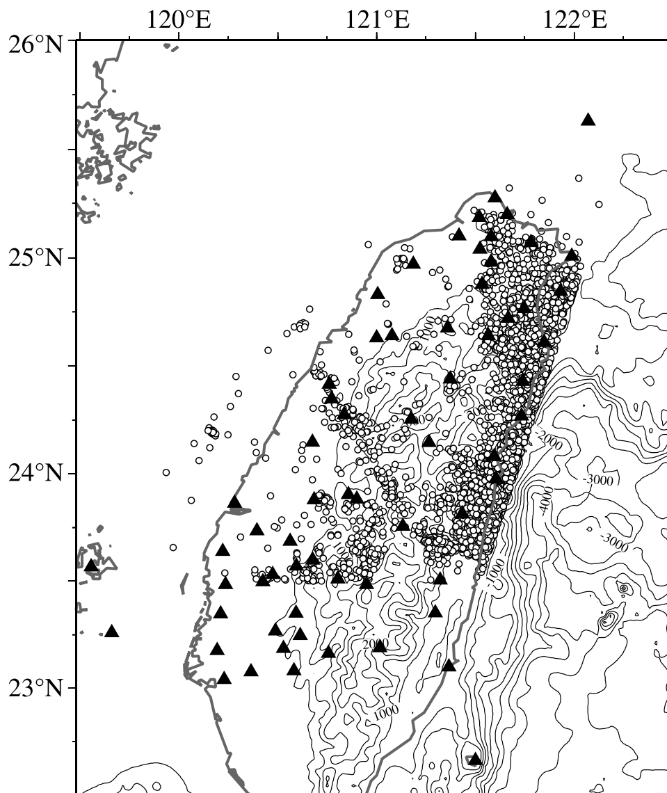
Figure 2. Location of seismic recording stations (triangles) and earthquakes (circles) used in this study.
