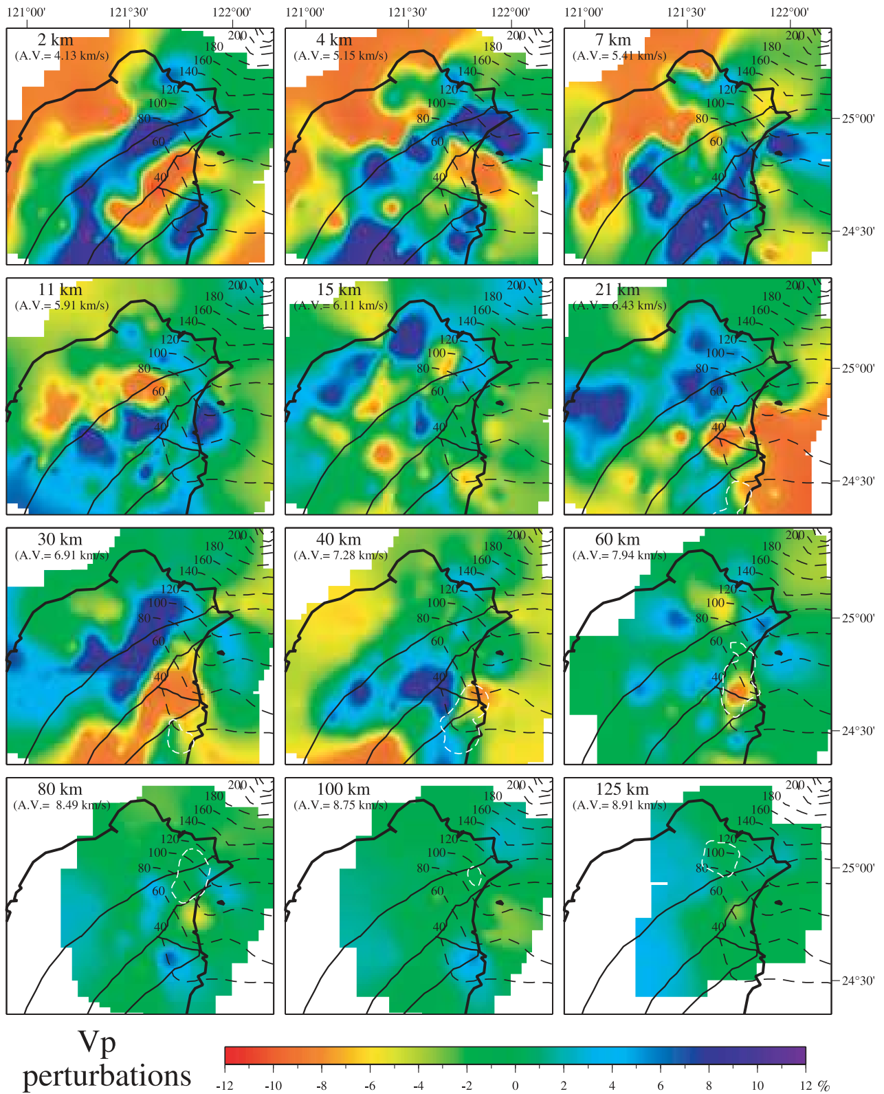
Figure 4. V_p tomography results displayed for 12 horizontal slices from 2 to 125 km. V_p values are in percentages with respect to the average P wave velocity at the depth of the slice. The black dashed lines represent the isobaths of the Wadati-Benioff zone [Font et al., 1999]. The white dashed lines represent the location of V_p/V_s anomalies larger than 1.78 (pasted from Figure 6).
