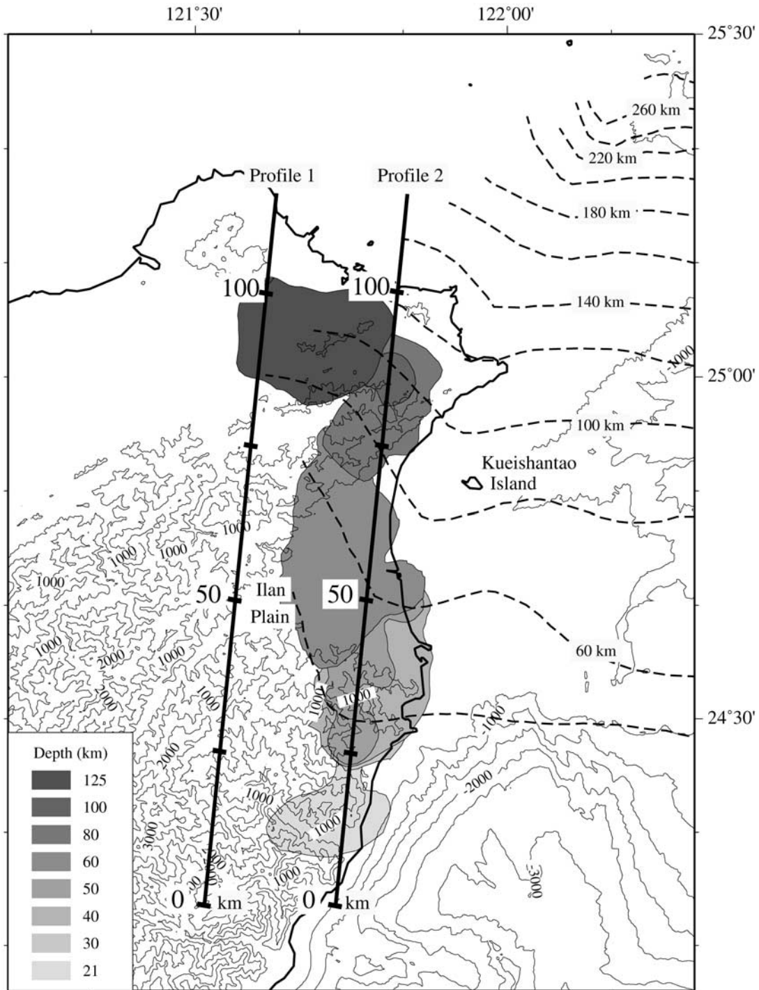
Figure 8. Geographical distribution of V_p/V_s values higher than 1.78, extracted from slices of Figure 6 and ranging from 21 km (light gray) to 125 km (dark gray). Dashed lines are isobaths of the Wadati-Benioff zone [Font et al. , 1999]. The areas of high V_p/V_s anomalies are located above the western edge of the Ryukyu slab. Tomographic profiles 1 and 2 are displayed in Figure 9.
