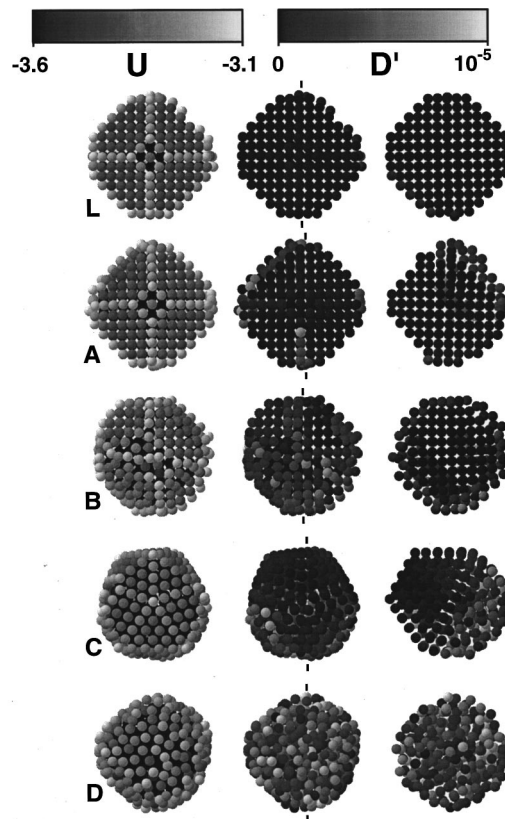
FIG. 11. Cluster configuration/property plots for \text{Au}_{459} at selected stages of its thermal evolution [ L , A , B , C , and D ; see Fig. 1(c)]. Configuration/energy plots (with shading following the potential energy scale, in eV, shown at the top) are displayed in the first column and configuration/diffusion plots in the two other columns. The configurations in the first and second columns correspond to a view of the \text{Au}_{459} cluster shown in Fig. 1 along a normal to the page [i.e., normal to the (100) front facet of the cluster]. The configuration on the right was obtained via the planar cut and rotation described in the caption to Fig. 10 (the cut line is indicated in the second column). An expanded color version of this figure, including the CNA signature, can be found as Fig. 2 in Ref. 20.
