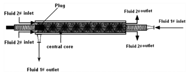
Fig. 2. Axial helically wound module.
