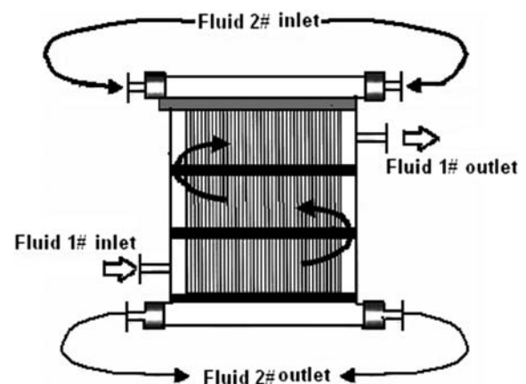
Fig. 5. Partially baffled rectangular module.
