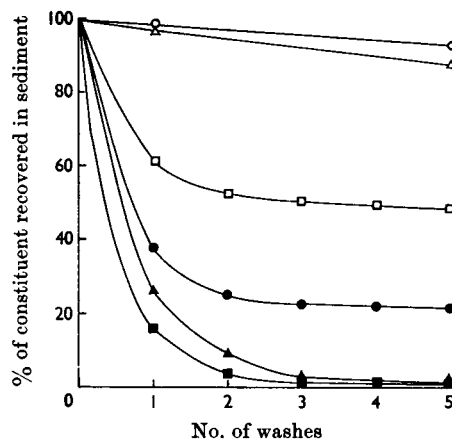
Fig. 1. Effect of repeated washing on distribution of chromaffin granule constituents between the soluble lysate and insoluble residue. Chromaffin granules were suspended in hypo-osmotic buffer, frozen, thawed and centrifuged, five times in all, as described in the Methods section. The ordinate gives the percentage of the amount of each constituent in the original suspension that was recovered in the five sediments. ○, Cytochrome b-559; △, phospholipids and cholesterol; □, dopamine β-hydroxylase activity; ●, total protein; ▲, chromogranin A; ■, catecholamines.
