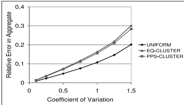
Figure 9: Aggregation error vs. population variance, UC frequency-based model, Z = 2 , \mu = 100 , Memory=10%
