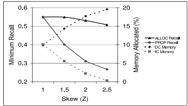
Figure 10: Memory allocation across joins: frequency-based model, Memory=20%
