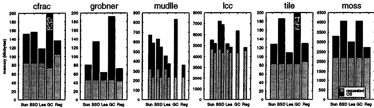
Figure 8: Memory overhead.
