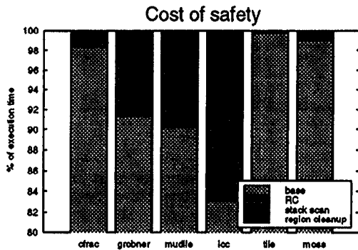
Figure 11: Region costs.
