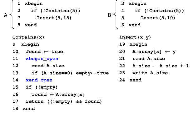
FIGURE 4: Flawed implementation of a table data structure with two methods, Contains(x) and Insert(x,y) . Although each method individually appears atomic, transactions A and B , which call those methods, may not appear atomic. In particular, the ordering \langle 1, 2, 3, 4, 5, 6, 7, 8 \rangle is allowed.
