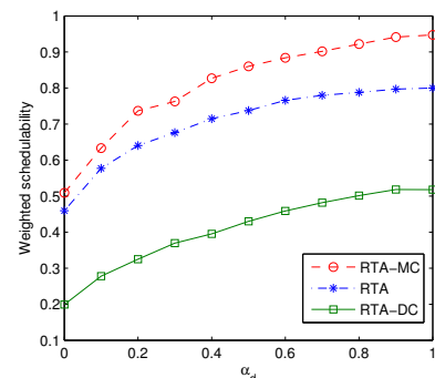
Figure 7: Experiments varying \alpha_d , with f_{mc} = 0.1 , and n = 8 .
