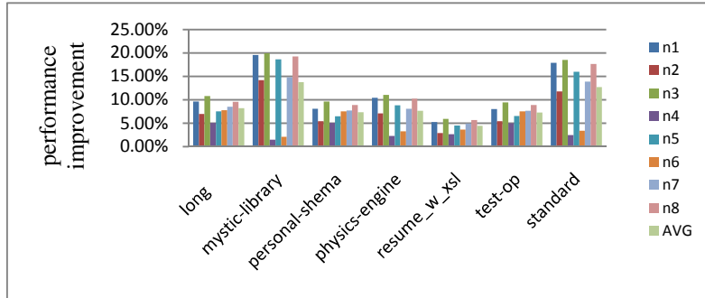
Fig. 6. Performance improvement for DOM parsing
