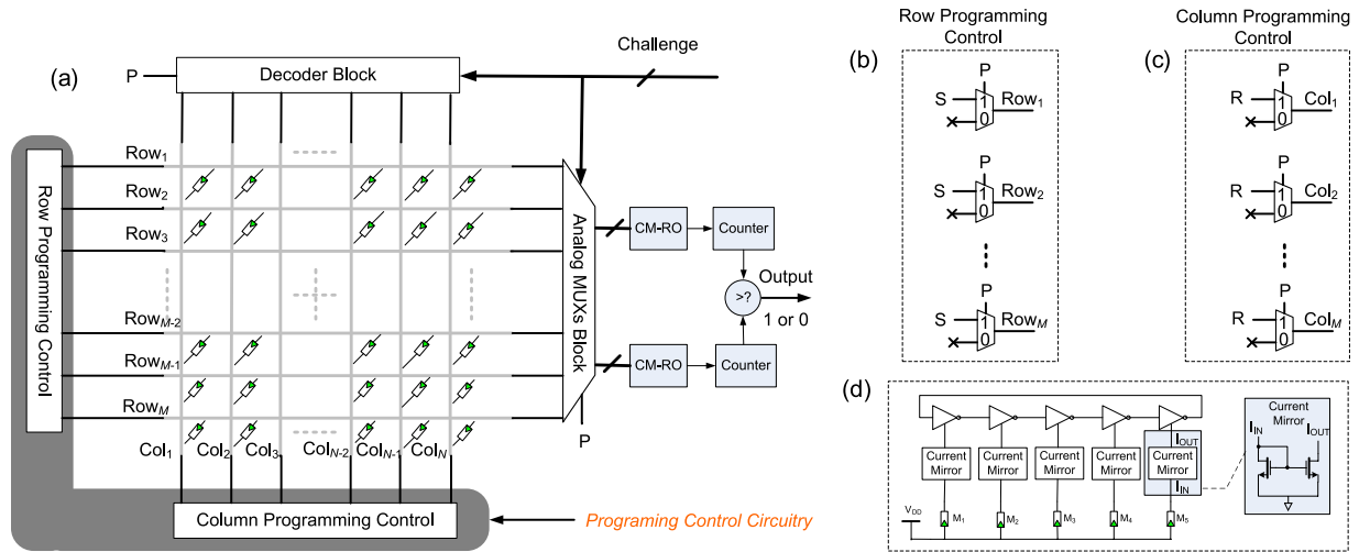
Figure 4. mrSPUF architecture. (a) Simplified mrSPUF architecture. All the memristors are in the ON state. The shaded programming control circuit comprises of the row programming control circuitry in (b) and column programming control circuitry in (c) which is employed to program memristors in nanocrossbar array before it acts as a PUF and facilitates reconfigurability of mrSPUF by subsequent reprogramming to refresh CRPs of mrSPUF to transform it into a new PUF instance. In contrast to the programming control circuit, the top decoder block and left analog multiplexers block, CM-ROs and counters enables the stimulation by a challenge and the extraction of a corresponding response. A challenge encoded as a vector of binary values (bits) is used to provide the address bits for both the analog multiplexers block and the decoder block. (d) CM-RO. Each current mirror starves only an inverter in the RO structure, where the bias memristor for each current mirror, M_i , is selected from the nanocrossbar array. Although variation in the oscillation frequency of each RO is slight influenced by the threshold voltage variation in the CMOS transistor composing the starved inverter and current mirror structures, the overall variation in the oscillation frequency is primarily determined by the variations in memristance of M_i if the supply voltage, V_{DD} , is kept constant.
