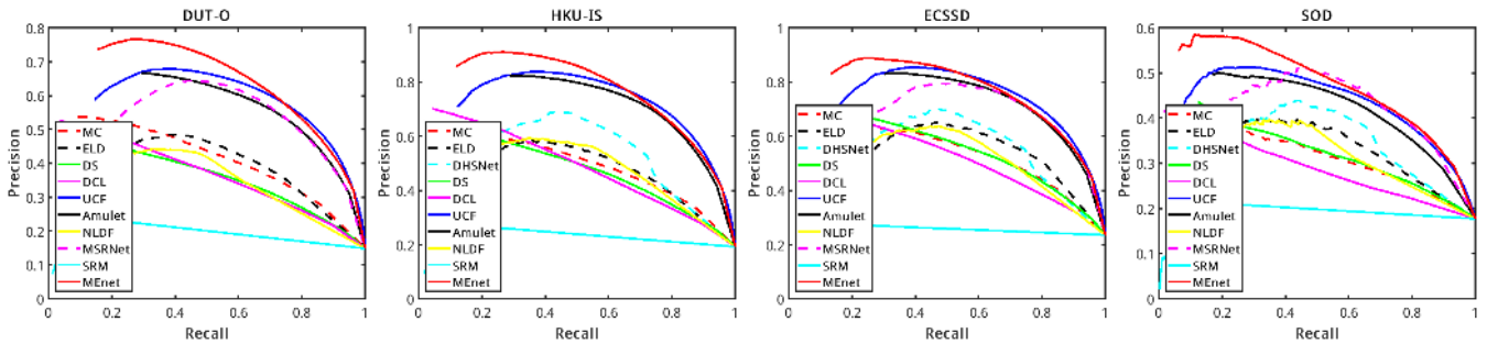
Figure 5: Comparison of precision-recall curves of other CNN-based methods on four datasets corrupted by AWGN (with random strengths).
