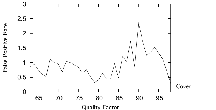
Figure 2. False positive rate in percents for the multi-classifiers trained for each JPEG quality factor.
