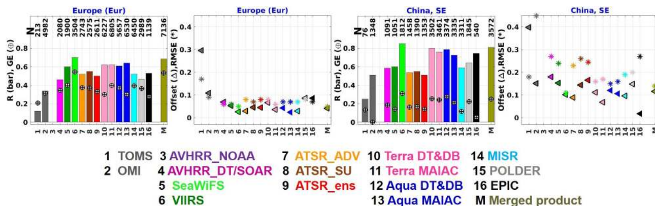
Figure 3. AERONET evaluation statistics for Europe and ChinaSE: correlation coefficient R , bar, and fraction of pixels satisfying the GCOS requirements, GE, \oplus ; offset (satellite product–AERONET), \Delta , and root-mean-square error RMSE, * . Shown for AOD monthly aggregates for each product (1 : 16; legend for products below the plot) and the L3 merged product (M; approach 2 with RM2 for all aerosol types; for details see Sect. 4.2) with corresponding colours (legend) for the selected regions (as in Fig. 1). N is the number of matches with AERONET. Note, for products that do not provide the global coverage (e.g. no retrieval over oceans), the results are missing. For all studied regions, see Fig. S7.
