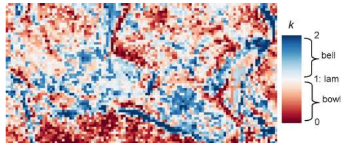
Fig. 6. Minnaert- k parameter obtained by RPV model inversion at 722 nm (lam = Lambertian).
