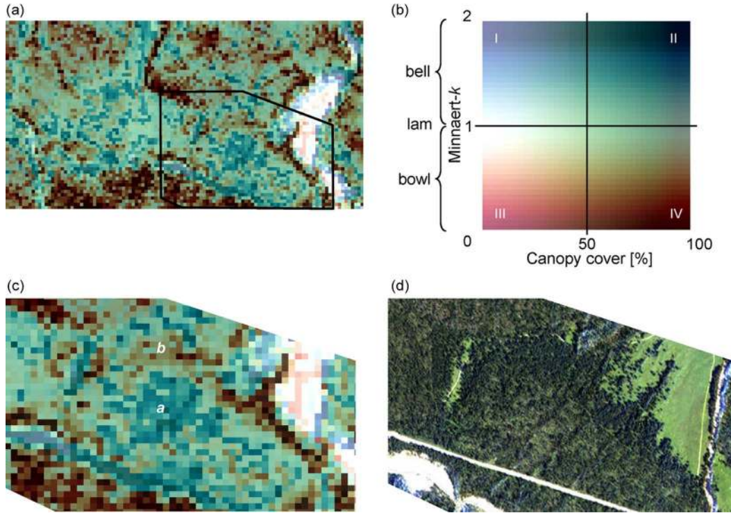
Fig. 8. (a) RGB result of merging the Minnaert- k map with the canopy cover map ( x -axis) and the color bar of the Minnaert- k map ( y -axis) ( \text{lam} = \text{Lambertian} ). (c) Zoom-in of the merged map as presented in panel A. (d) The reference image as derived from a high resolution stereo camera (HRSC) acquisition in summer 2003 (true color).
