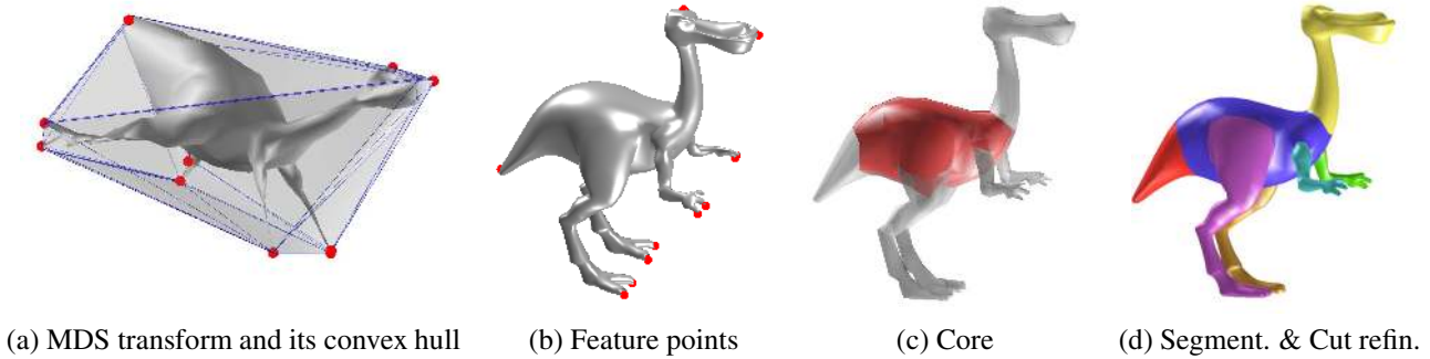
Figure 2. Algorithm [14] outline.
