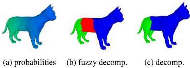
Figure 1. Algorithm [15] outline.
