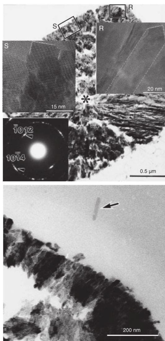
Figure 12. Hematite ( \alpha Fe 2 O 3 ) mesocrystals: top: Transmission electron micrograph of a thin section together with HRTEM pictures of areas S and R as insets. The * notes the position where the electron diffraction data (shown in the lower inset) was taken. Bottom: TEM micrograph of a thin section of a pseudocubic particle. An arrow indicates a subcrystal separated from the solution. Figure reproduced from ref. [59] with permission of Academic Press.
