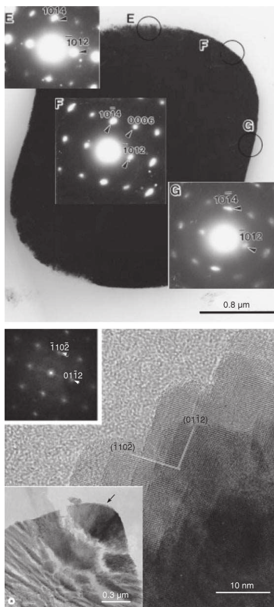
Figure 11. Hematite ( \alpha Fe 2 O 3 ) mesocrystals: top: Transmission electron micrograph of a thin section and electron diffraction patterns obtained from the parts E, F, and G. Bottom: inset lower left is the transmission electron micrograph of a section around a corner of a pseudocubic particle; main photo: High resolution electron micrograph of the area indicated by an arrow in the lower left inset. Upper left inset is the Fourier diffractogram of the lower inset. Figure reproduced from ref. [59] with permission of Academic Press.
